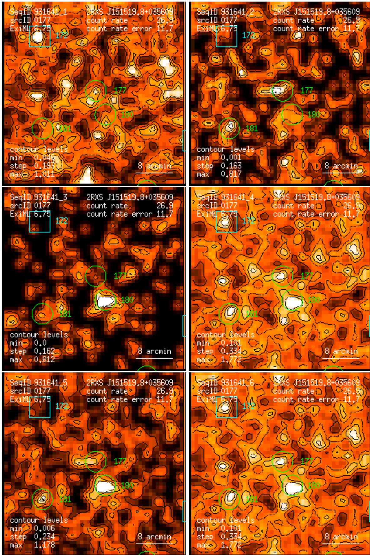
Figure 177: RASS 931641: detection 0177: band rate images, Gaussian filter: (1) PSPC channels 11 – 41, (2) 52 – 90, (3) 91 – 201, (4) 11 – 235, (5) 52 – 201, (6) 11 – 201. Broad band rates in counts/ks. Band rate contour levels in counts/ks/arcmin 2 .
