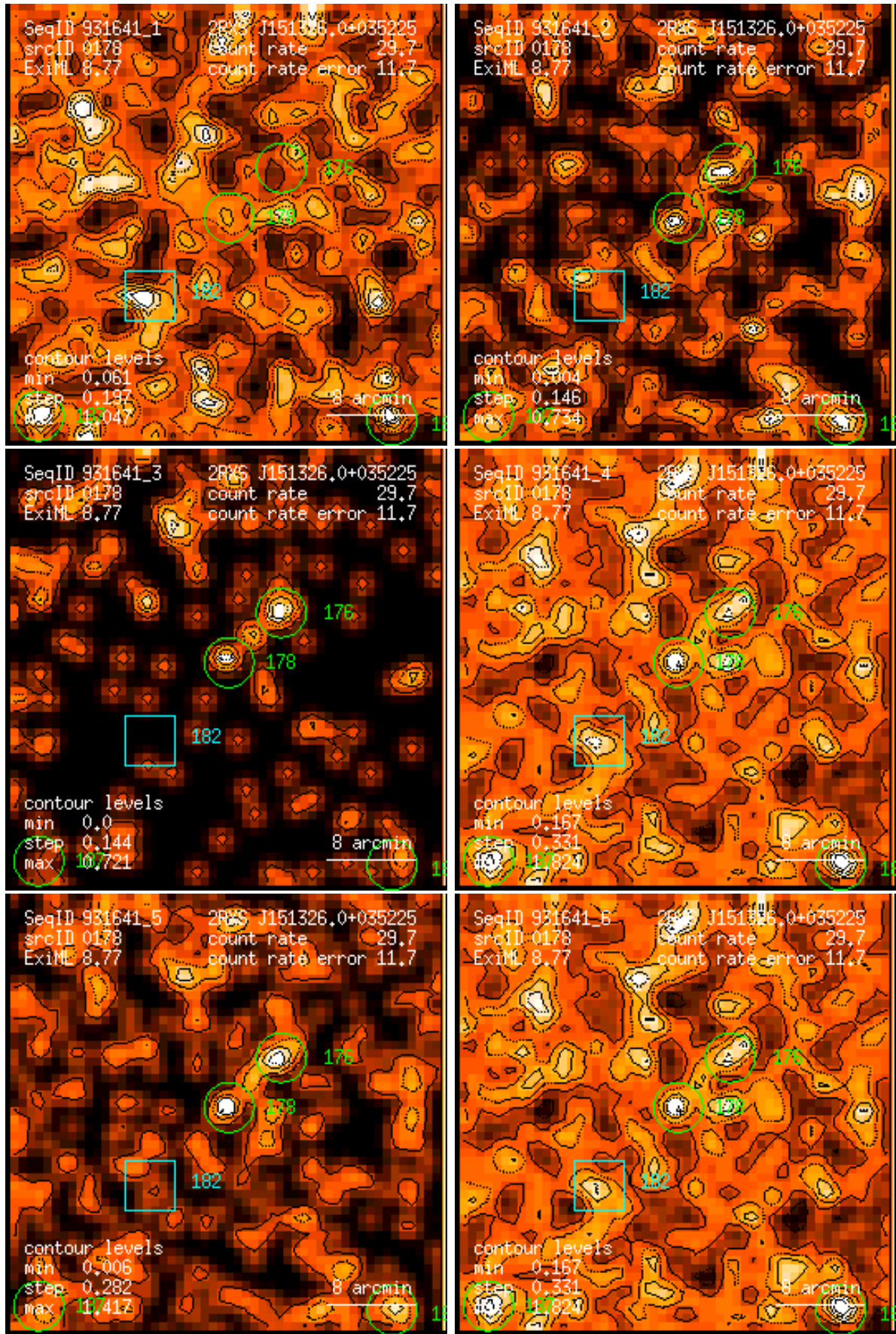
Figure 178: RASS 931641: detection 0178: band rate images, Gaussian filter: (1) PSPC channels 11 – 41, (2) 52 – 90, (3) 91 – 201, (4) 11 – 235, (5) 52 – 201, (6) 11 – 201. Broad band rates in counts/ks. Band rate contour levels in counts/ks/arcmin 2 .
