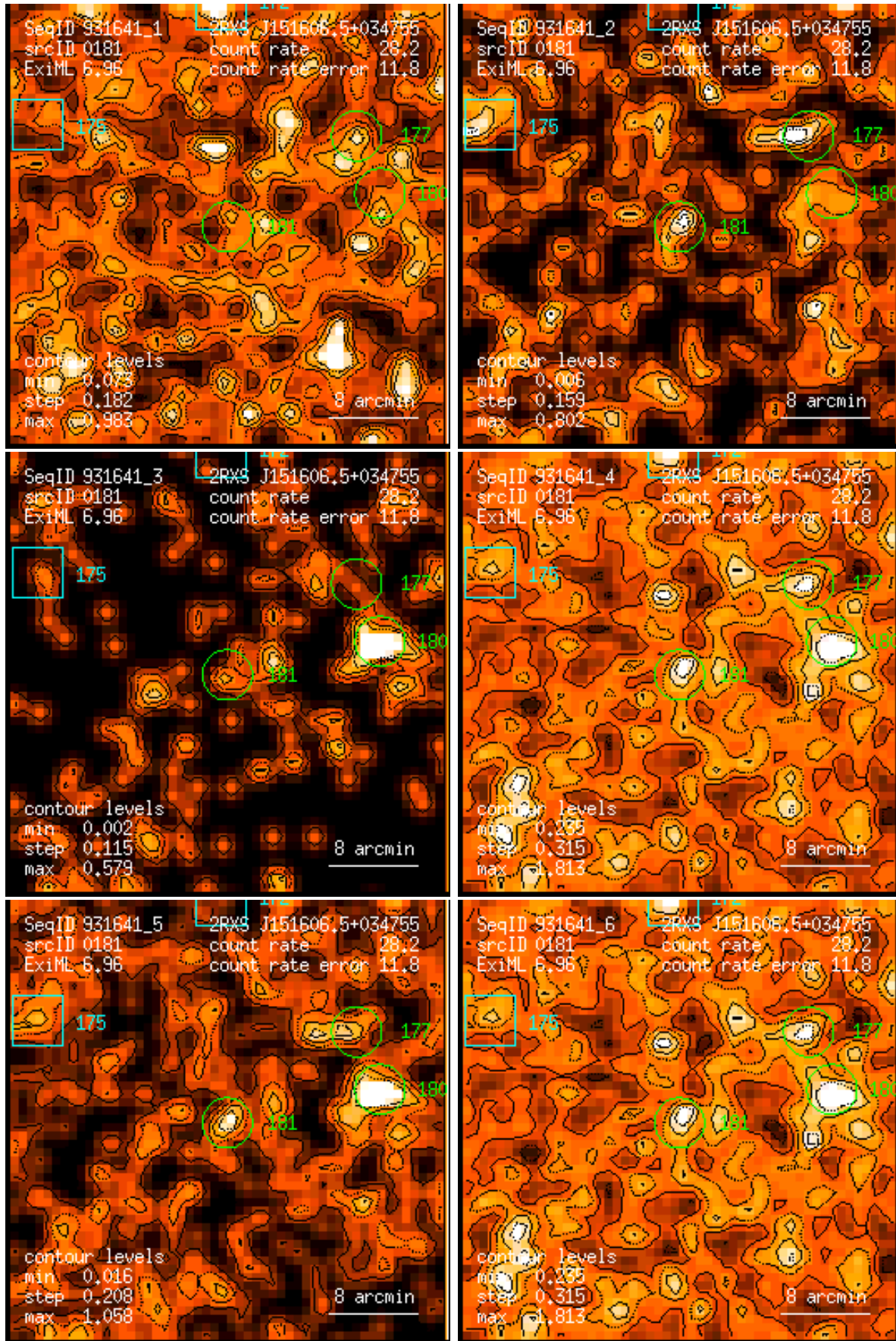
Figure 181: RASS 931641: detection 0181: band rate images, Gaussian filter: (1) PSPC channels 11 – 41, (2) 52 – 90, (3) 91 – 201, (4) 11 – 235, (5) 52 – 201, (6) 11 – 201. Broad band rates in counts/ks. Band rate contour levels in counts/ks/arcmin 2 .
