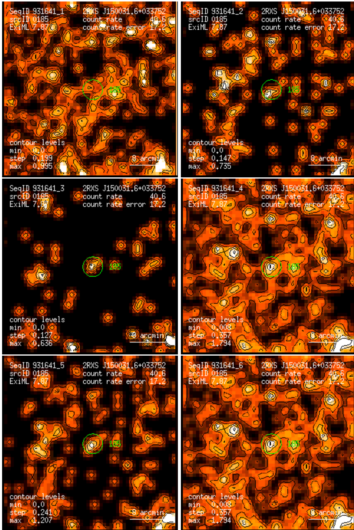
Figure 185: RASS 931641: detection 0185: band rate images, Gaussian filter: (1) PSPC channels 11 – 41, (2) 52 – 90, (3) 91 – 201, (4) 11 – 235, (5) 52 – 201, (6) 11 – 201. Broad band rates in counts/ks. Band rate contour levels in counts/ks/arcmin 2 .
