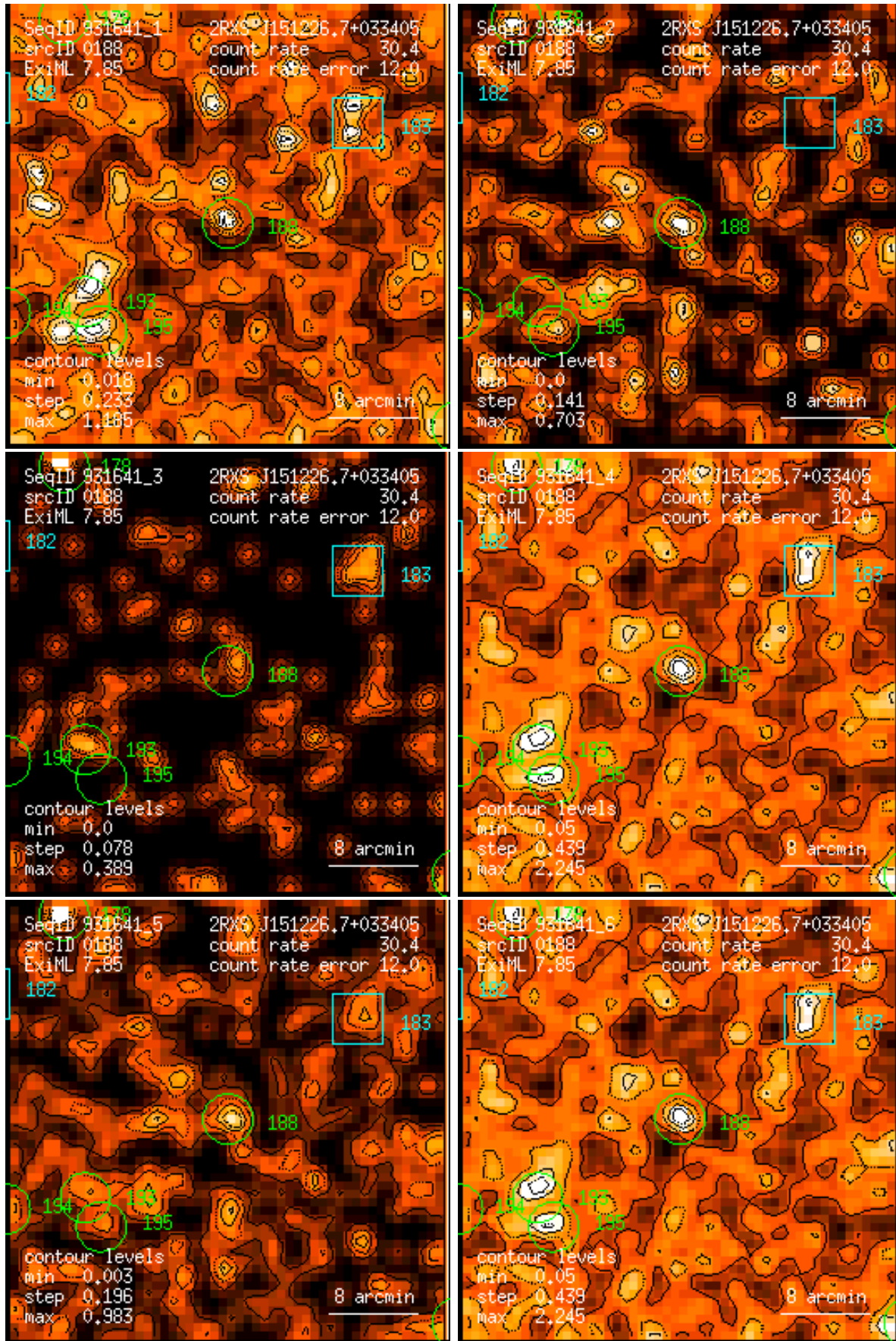
Figure 188: RASS 931641: detection 0188: band rate images, Gaussian filter: (1) PSPC channels 11 – 41, (2) 52 – 90, (3) 91 – 201, (4) 11 – 235, (5) 52 – 201, (6) 11 – 201. Broad band rates in counts/ks. Band rate contour levels in counts/ks/arcmin 2 .
