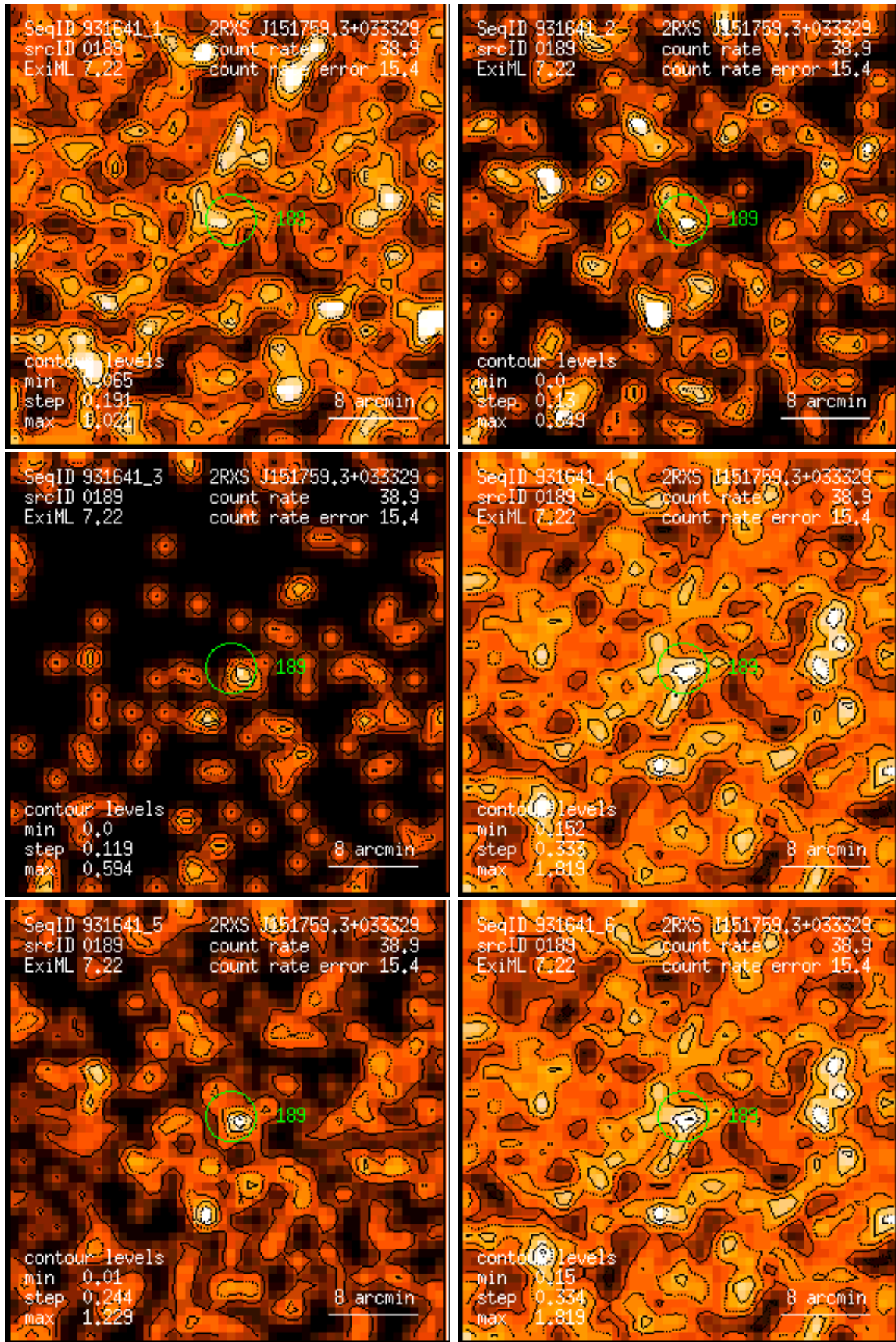
Figure 189: RASS 931641: detection 0189: band rate images, Gaussian filter: (1) PSPC channels 11 – 41, (2) 52 – 90, (3) 91 – 201, (4) 11 – 235, (5) 52 – 201, (6) 11 – 201. Broad band rates in counts/ks. Band rate contour levels in counts/ks/arcmin 2 .
