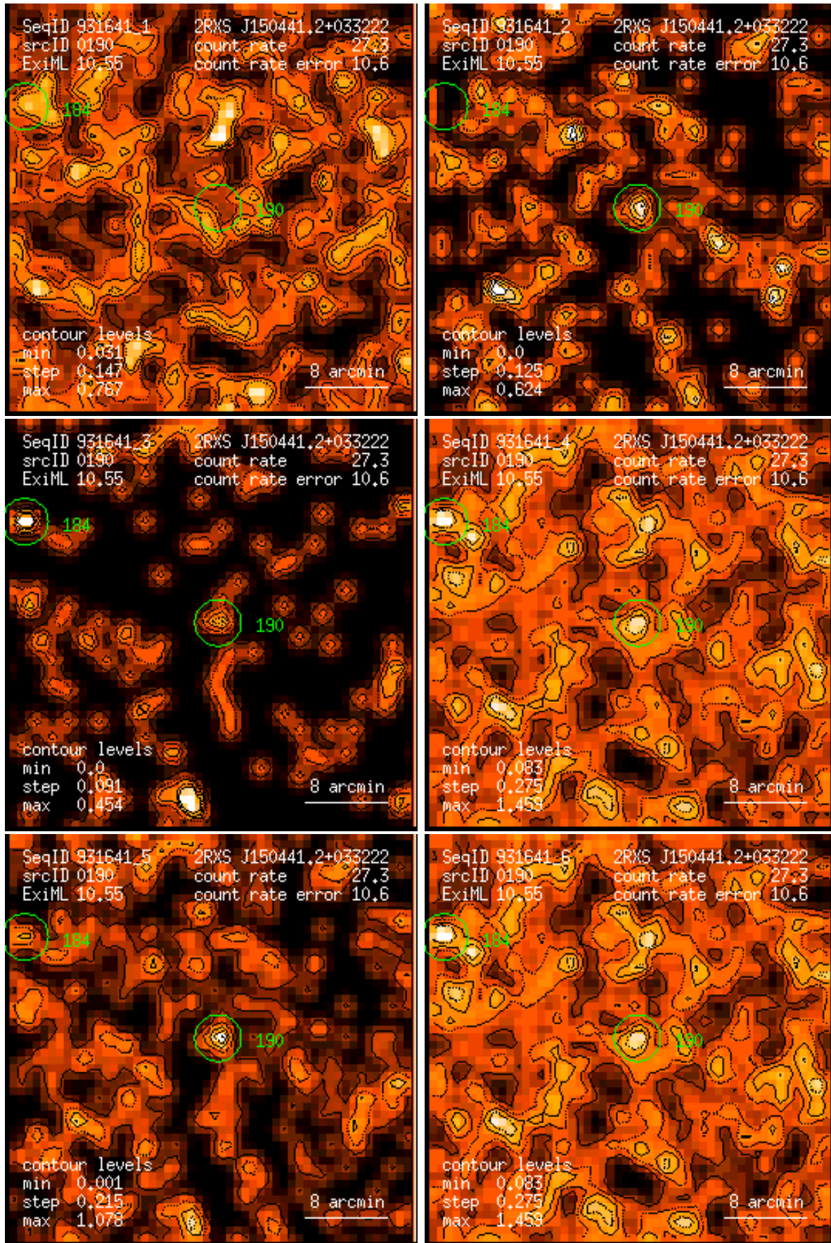
Figure 190: RASS 931641: detection 0190: band rate images, Gaussian filter: (1) PSPC channels 11 – 41, (2) 52 – 90, (3) 91 – 201, (4) 11 – 235, (5) 52 – 201, (6) 11 – 201. Broad band rates in counts/ks. Band rate contour levels in counts/ks/arcmin 2 .
