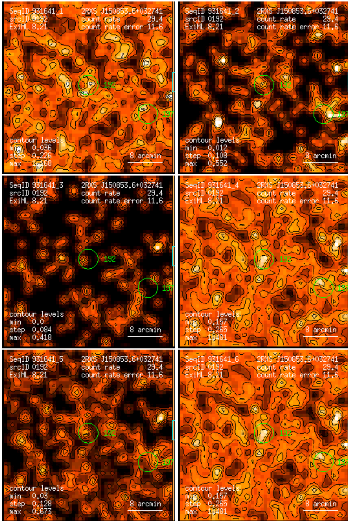
Figure 192: RASS 931641: detection 0192: band rate images, Gaussian filter: (1) PSPC channels 11 – 41, (2) 52 – 90, (3) 91 – 201, (4) 11 – 235, (5) 52 – 201, (6) 11 – 201. Broad band rates in counts/ks. Band rate contour levels in counts/ks/arcmin 2 .
