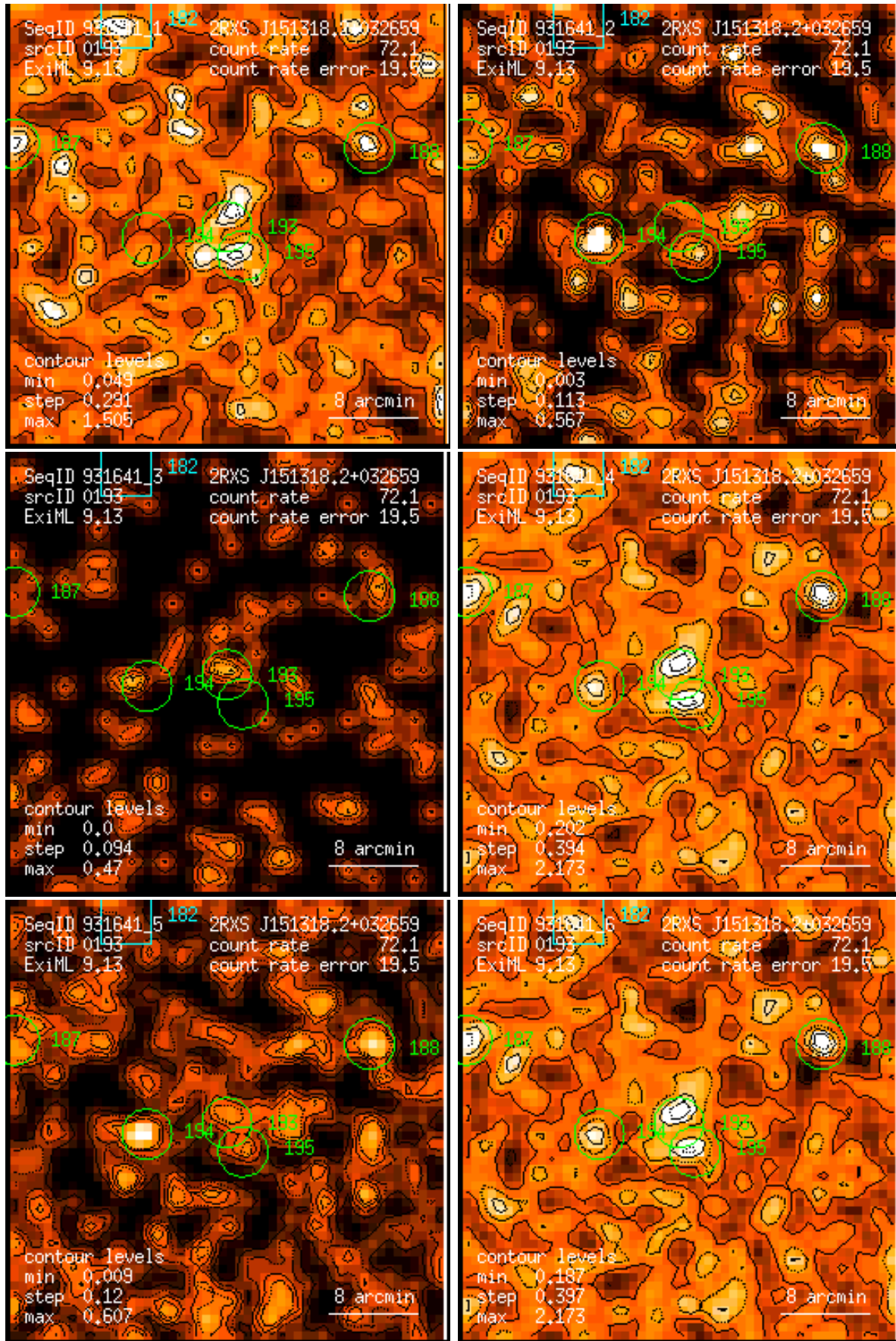
Figure 193: RASS 931641: detection 0193: band rate images, Gaussian filter: (1) PSPC channels 11 – 41, (2) 52 – 90, (3) 91 – 201, (4) 11 – 235, (5) 52 – 201, (6) 11 – 201. Broad band rates in counts/ks. Band rate contour levels in counts/ks/arcmin 2 .
