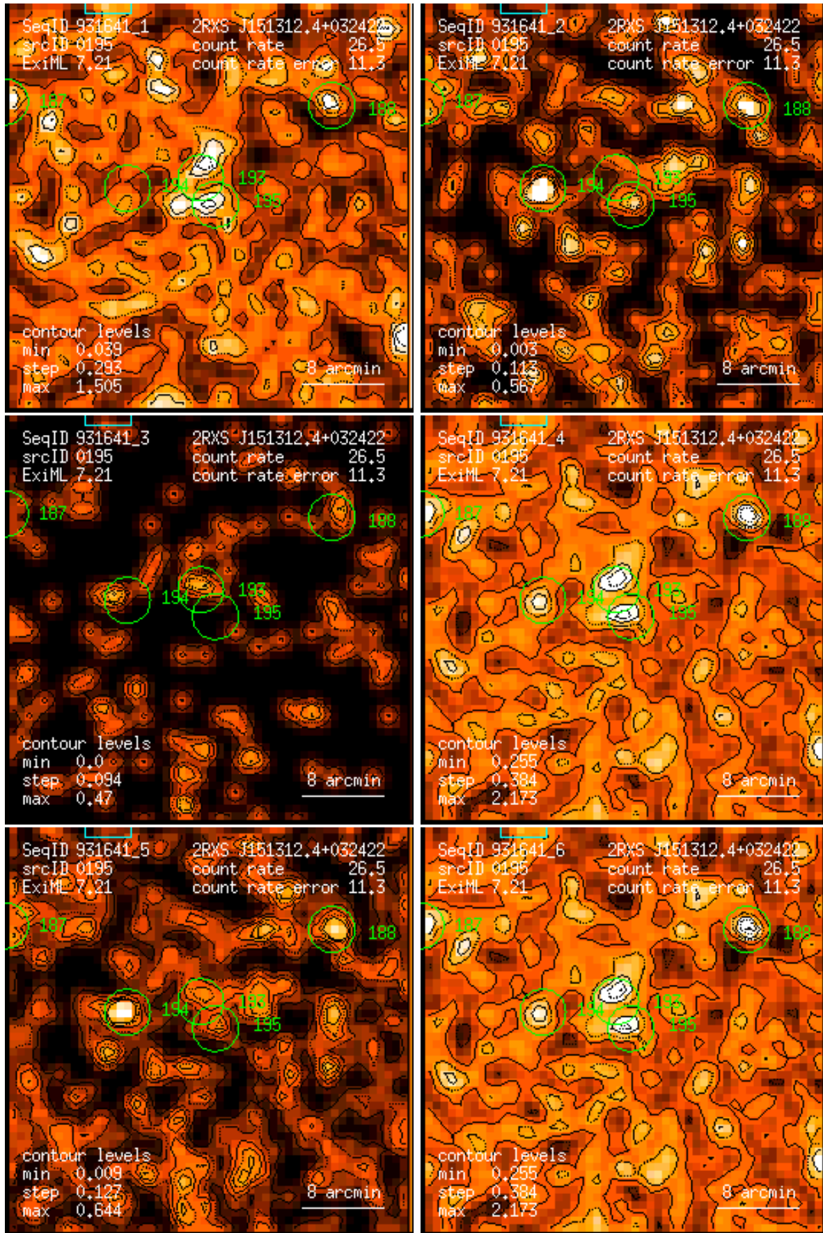
Figure 195: RASS 931641: detection 0195: band rate images, Gaussian filter: (1) PSPC channels 11 – 41, (2) 52 – 90, (3) 91 – 201, (4) 11 – 235, (5) 52 – 201, (6) 11 – 201. Broad band rates in counts/ks. Band rate contour levels in counts/ks/arcmin 2 .
