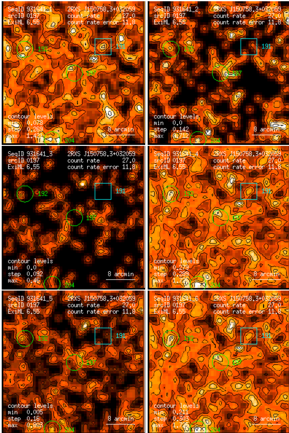
Figure 197: RASS 931641: detection 0197: band rate images, Gaussian filter: (1) PSPC channels 11 – 41, (2) 52 – 90, (3) 91 – 201, (4) 11 – 235, (5) 52 – 201, (6) 11 – 201. Broad band rates in counts/ks. Band rate contour levels in counts/ks/arcmin 2 .
