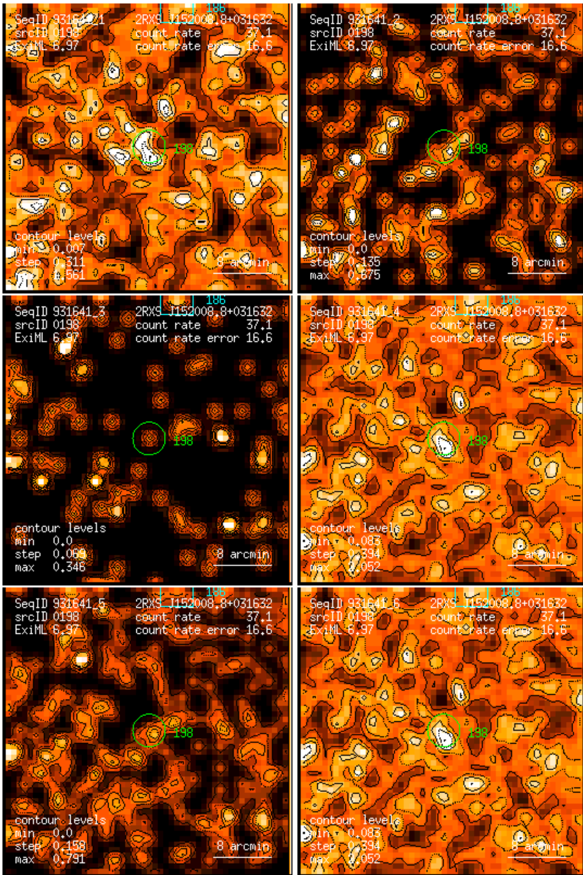
Figure 198: RASS 931641: detection 0198: band rate images, Gaussian filter: (1) PSPC channels 11 – 41, (2) 52 – 90, (3) 91 – 201, (4) 11 – 235, (5) 52 – 201, (6) 11 – 201. Broad band rates in counts/ks. Band rate contour levels in counts/ks/arcmin 2 .
