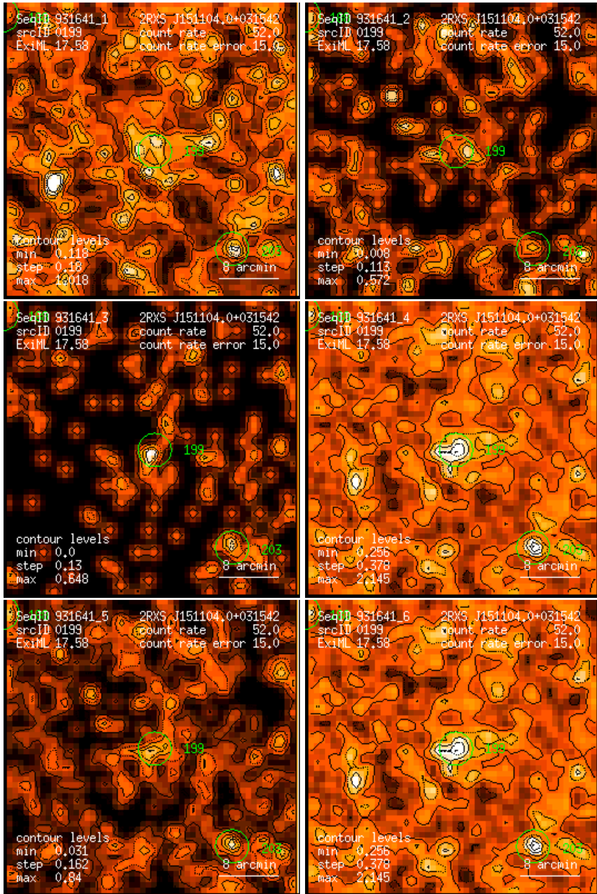
Figure 199: RASS 931641: detection 0199: band rate images, Gaussian filter: (1) PSPC channels 11 – 41, (2) 52 – 90, (3) 91 – 201, (4) 11 – 235, (5) 52 – 201, (6) 11 – 201. Broad band rates in counts/ks. Band rate contour levels in counts/ks/arcmin 2 .
