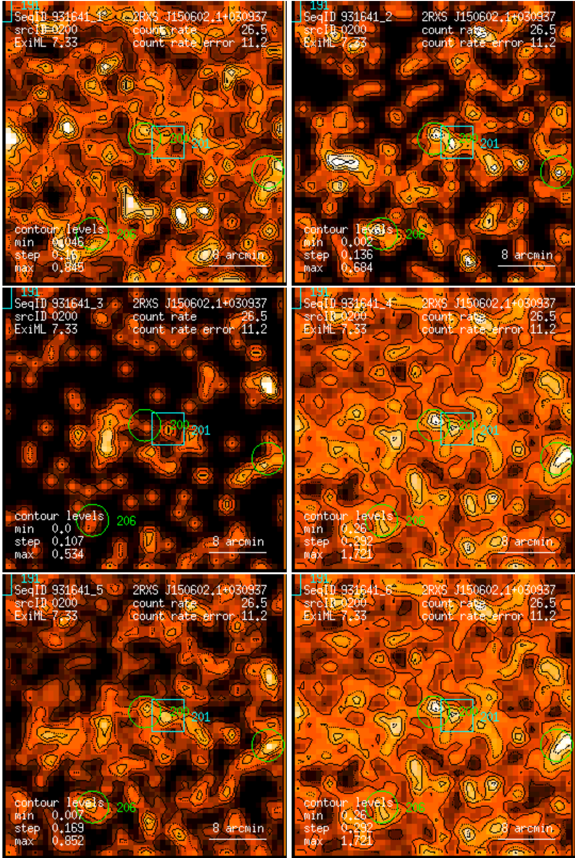
Figure 200: RASS 931641: detection 0200: band rate images, Gaussian filter: (1) PSPC channels 11 – 41, (2) 52 – 90, (3) 91 – 201, (4) 11 – 235, (5) 52 – 201, (6) 11 – 201. Broad band rates in counts/ks. Band rate contour levels in counts/ks/arcmin 2 .
