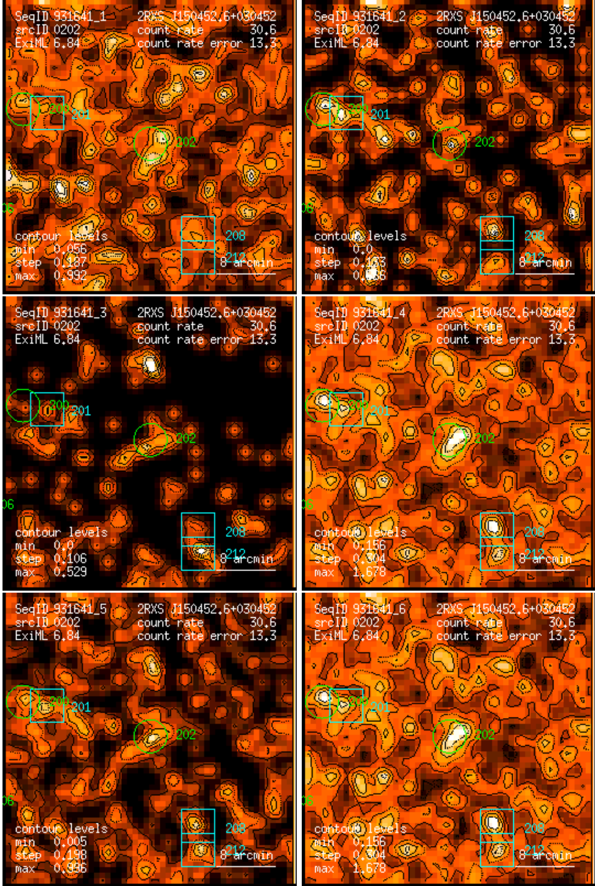
Figure 202: RASS 931641: detection 0202: band rate images, Gaussian filter: (1) PSPC channels 11 – 41, (2) 52 – 90, (3) 91 – 201, (4) 11 – 235, (5) 52 – 201, (6) 11 – 201. Broad band rates in counts/ks. Band rate contour levels in counts/ks/arcmin 2 .
