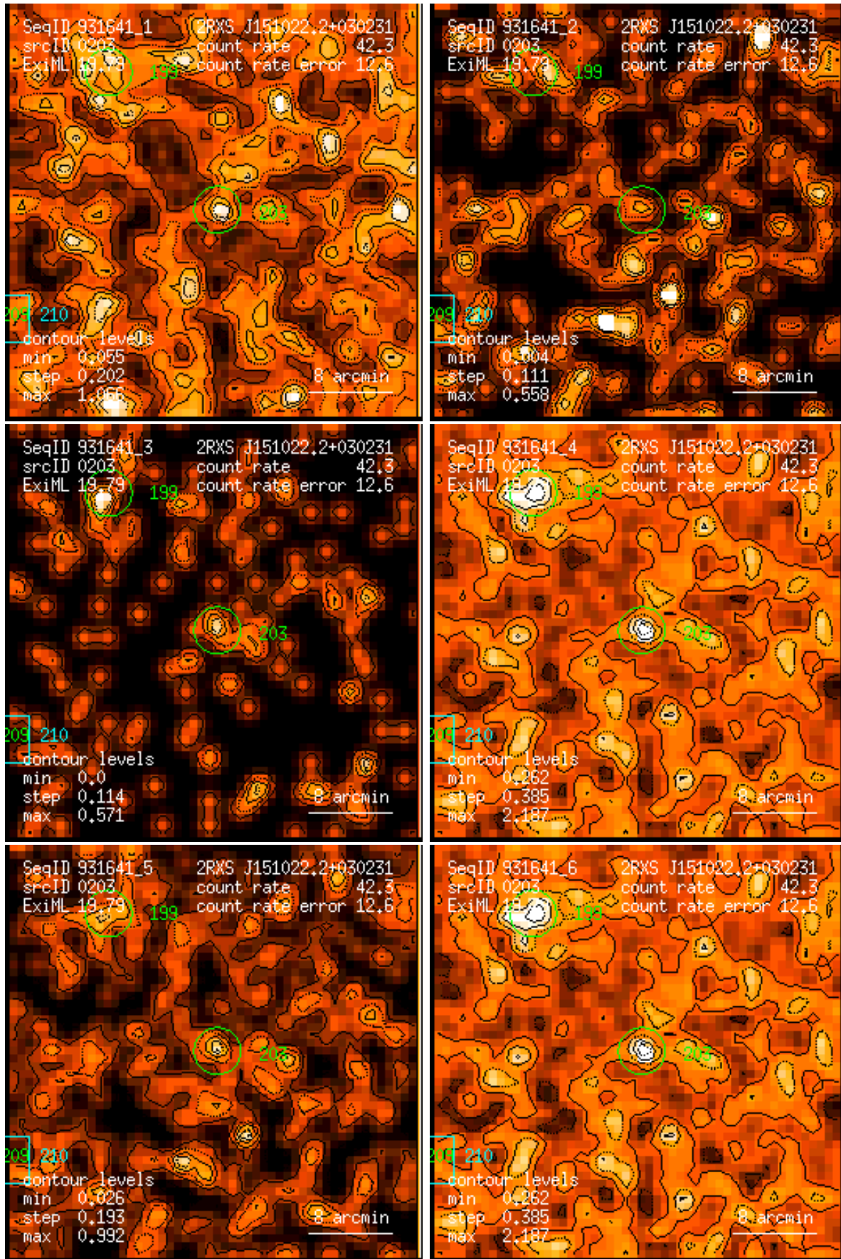
Figure 203: RASS 931641: detection 0203: band rate images, Gaussian filter: (1) PSPC channels 11 – 41, (2) 52 – 90, (3) 91 – 201, (4) 11 – 235, (5) 52 – 201, (6) 11 – 201. Broad band rates in counts/ks. Band rate contour levels in counts/ks/arcmin 2 .
