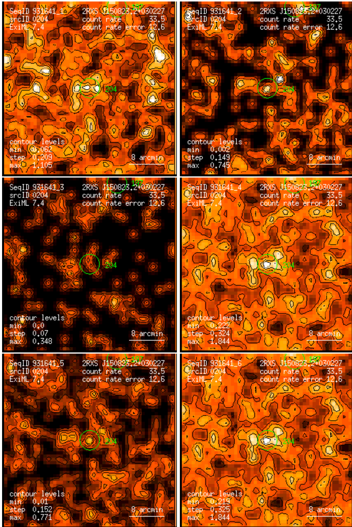
Figure 204: RASS 931641: detection 0204: band rate images, Gaussian filter: (1) PSPC channels 11 – 41, (2) 52 – 90, (3) 91 – 201, (4) 11 – 235, (5) 52 – 201, (6) 11 – 201. Broad band rates in counts/ks. Band rate contour levels in counts/ks/arcmin 2 .
