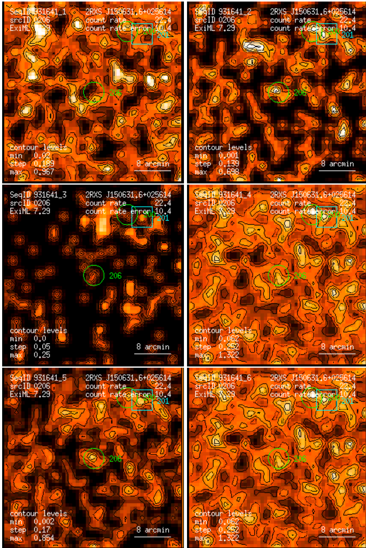
Figure 206: RASS 931641: detection 0206: band rate images, Gaussian filter: (1) PSPC channels 11 – 41, (2) 52 – 90, (3) 91 – 201, (4) 11 – 235, (5) 52 – 201, (6) 11 – 201. Broad band rates in counts/ks. Band rate contour levels in counts/ks/arcmin 2 .
