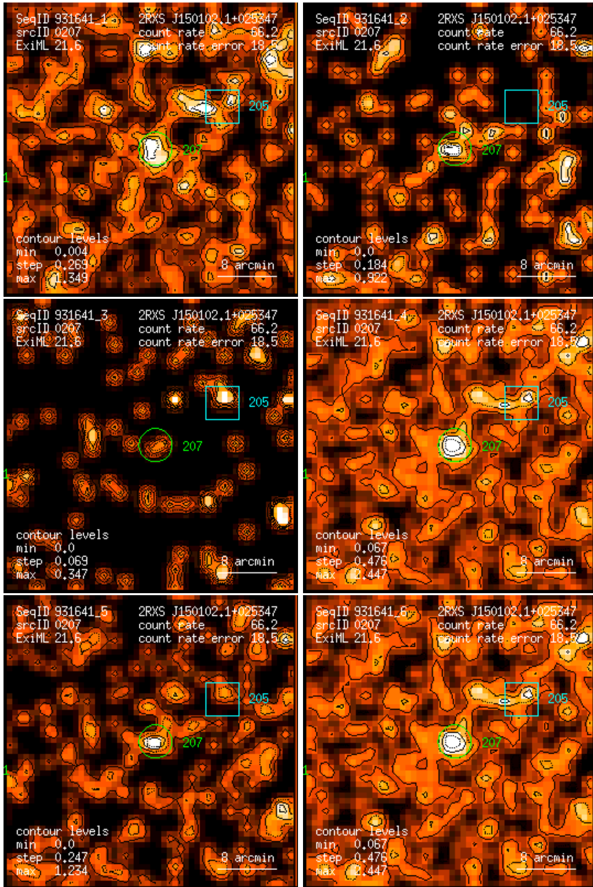
Figure 207: RASS 931641: detection 0207: band rate images, Gaussian filter: (1) PSPC channels 11 – 41, (2) 52 – 90, (3) 91 – 201, (4) 11 – 235, (5) 52 – 201, (6) 11 – 201. Broad band rates in counts/ks. Band rate contour levels in counts/ks/arcmin 2 .
