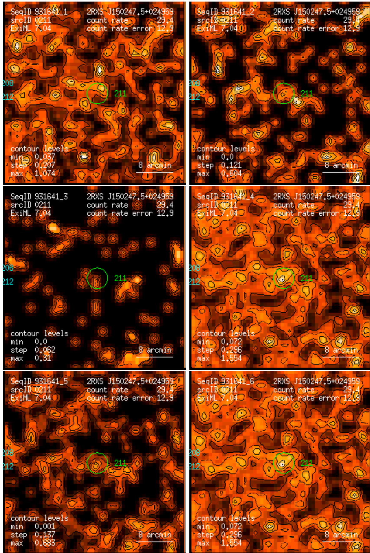
Figure 211: RASS 931641: detection 0211: band rate images, Gaussian filter: (1) PSPC channels 11 – 41, (2) 52 – 90, (3) 91 – 201, (4) 11 – 235, (5) 52 – 201, (6) 11 – 201. Broad band rates in counts/ks. Band rate contour levels in counts/ks/arcmin 2 .
