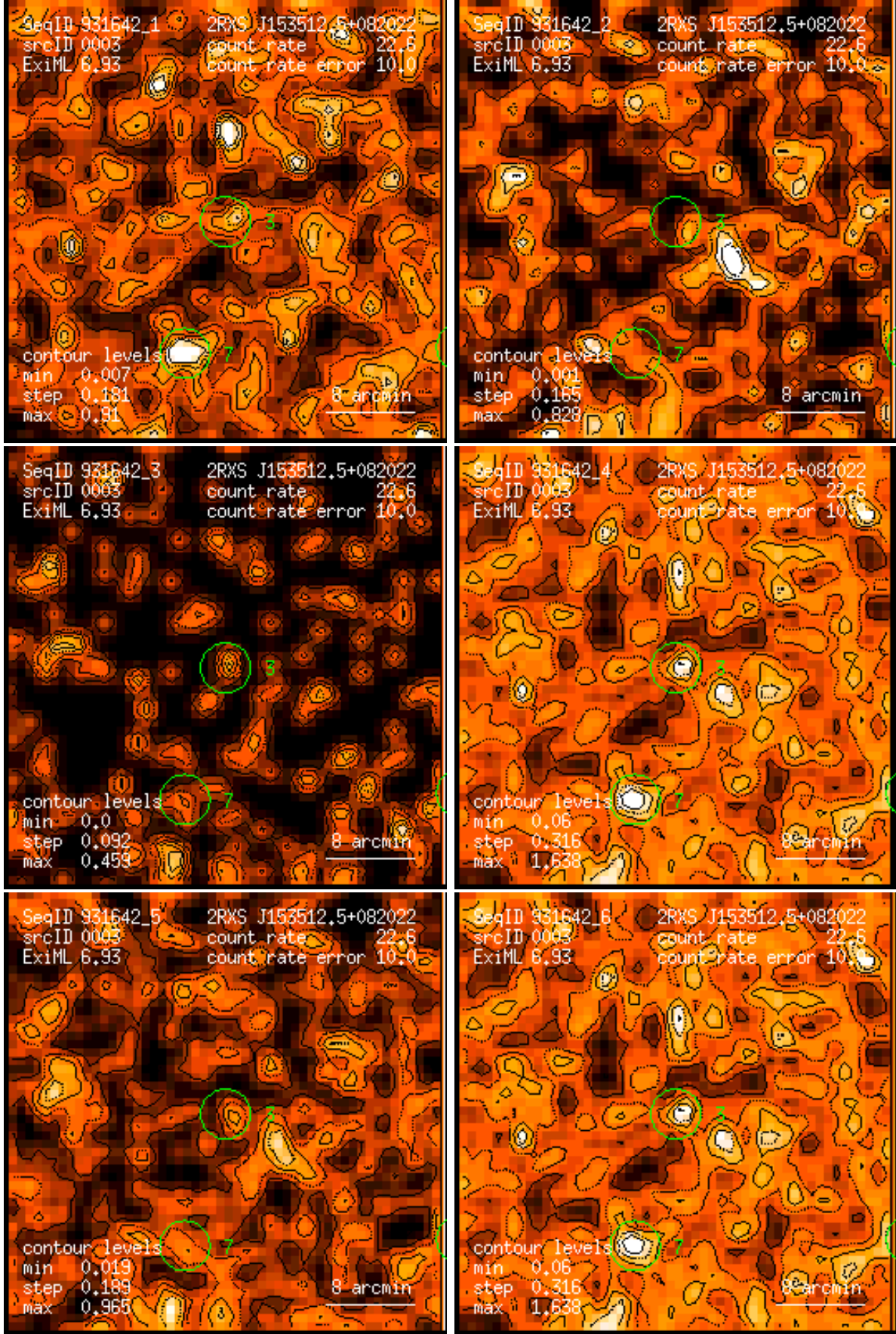
Figure 3: RASS 931642: detection 0003: band rate images, Gaussian filter: (1) PSPC channels 11 – 41, (2) 52 – 90, (3) 91 – 201, (4) 11 – 235, (5) 52 – 201, (6) 11 – 201. Broad band rates in counts/ks. Band rate contour levels in counts/ks/arcmin 2 .
