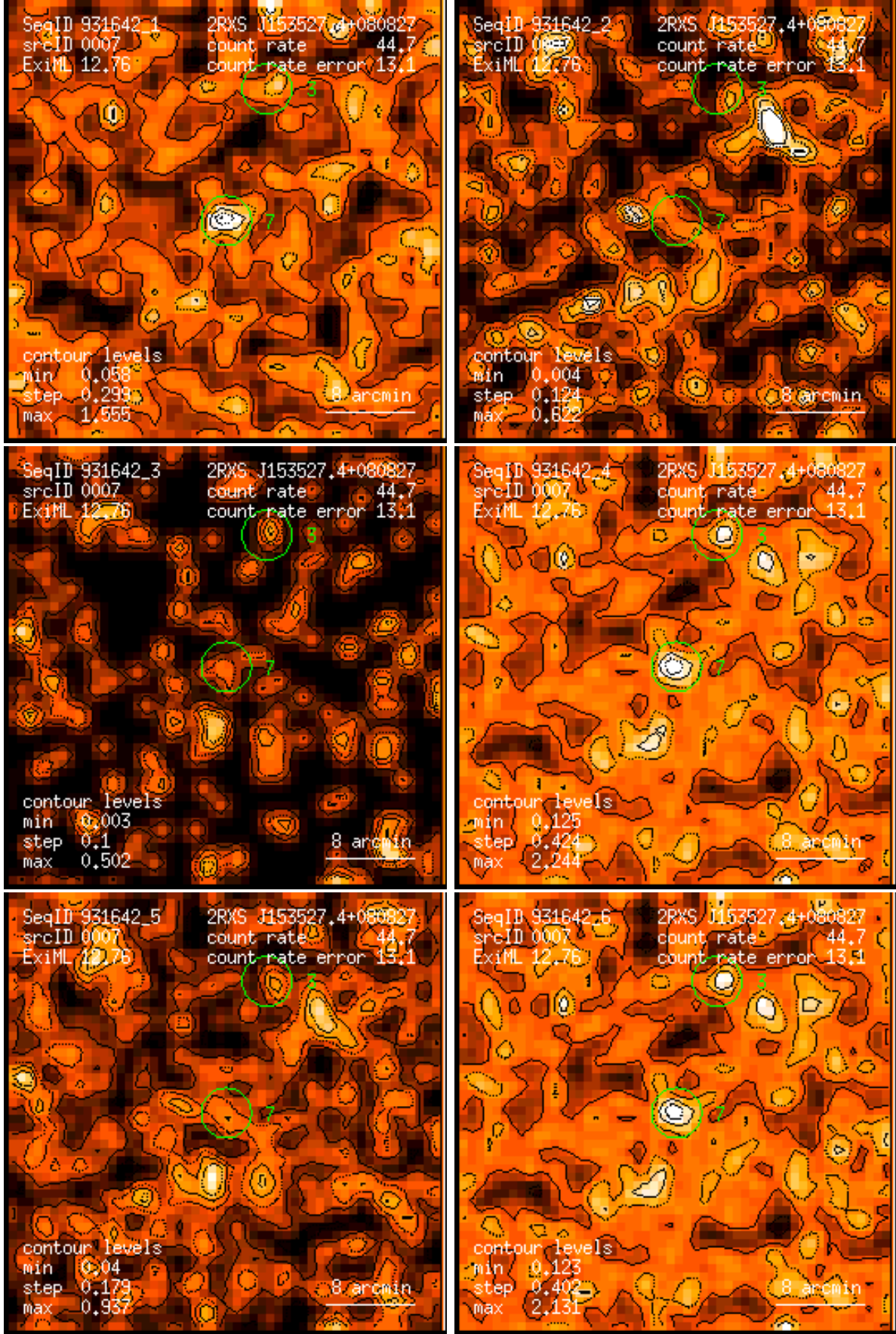
Figure 7: RASS 931642: detection 0007: band rate images, Gaussian filter: (1) PSPC channels 11 – 41, (2) 52 – 90, (3) 91 – 201, (4) 11 – 235, (5) 52 – 201, (6) 11 – 201. Broad band rates in counts/ks. Band rate contour levels in counts/ks/arcmin 2 .
