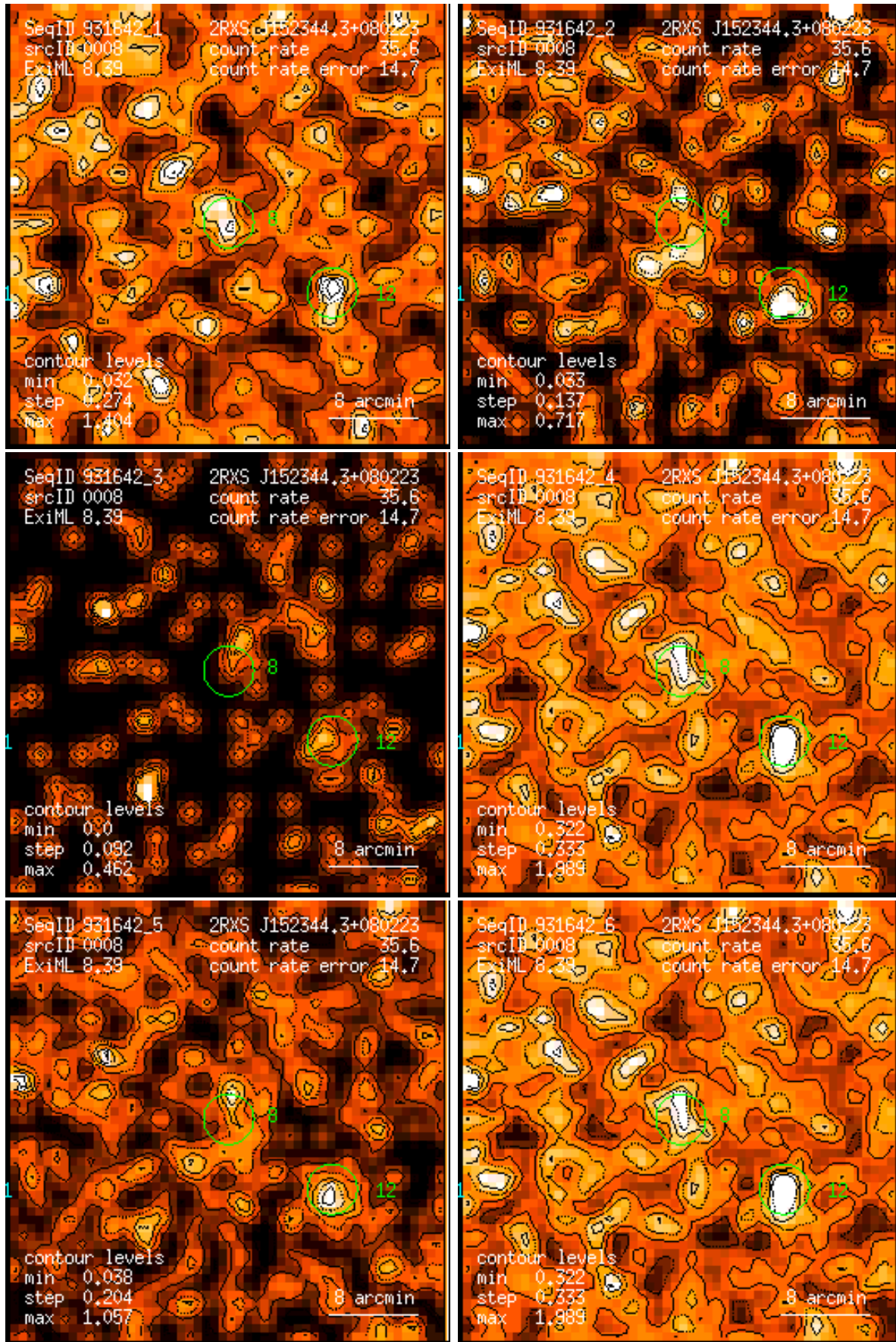
Figure 8: RASS 931642: detection 0008: band rate images, Gaussian filter: (1) PSPC channels 11 – 41, (2) 52 – 90, (3) 91 – 201, (4) 11 – 235, (5) 52 – 201, (6) 11 – 201. Broad band rates in counts/ks. Band rate contour levels in counts/ks/arcmin 2 .
