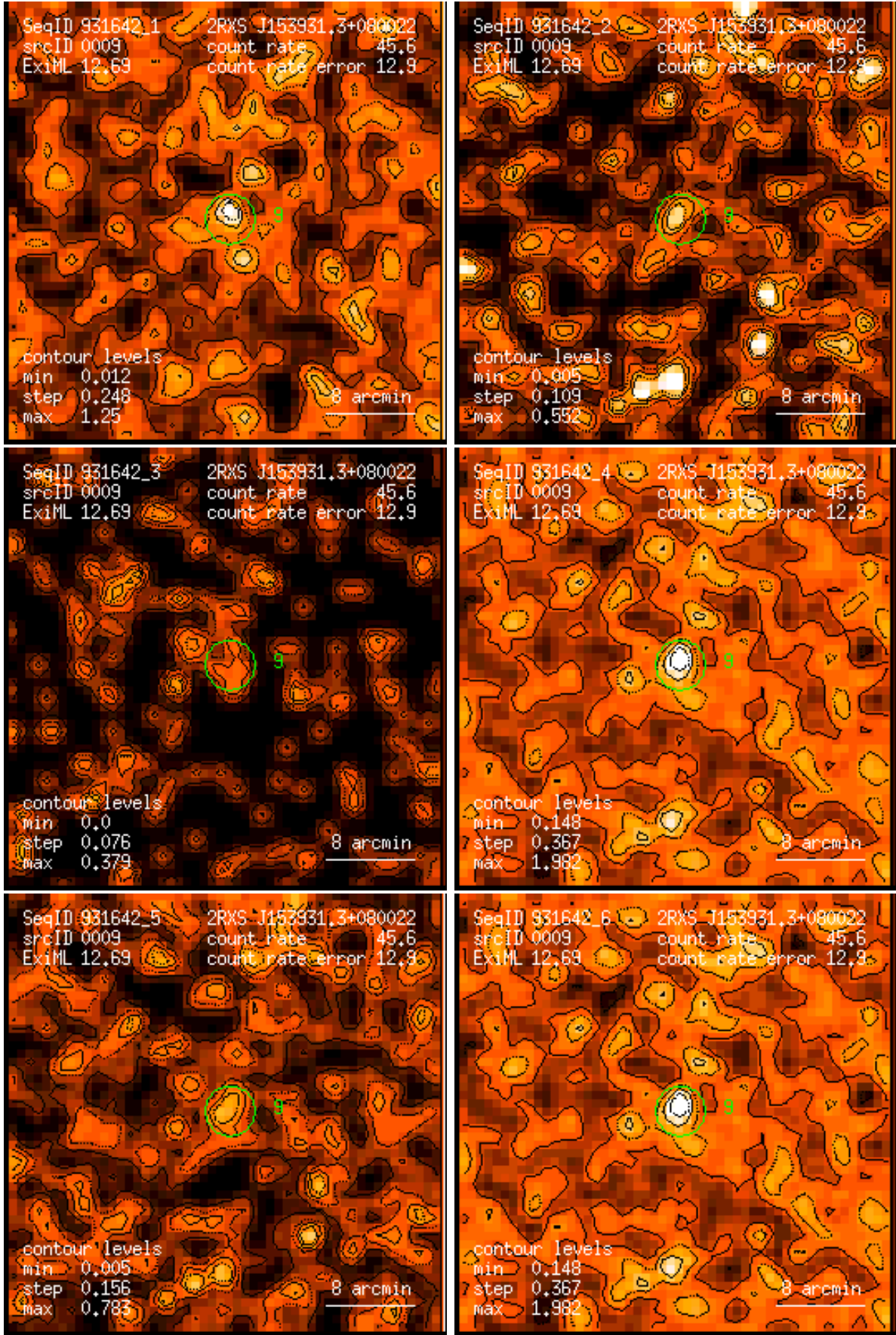
Figure 9: RASS 931642: detection 0009: band rate images, Gaussian filter: (1) PSPC channels 11 – 41, (2) 52 – 90, (3) 91 – 201, (4) 11 – 235, (5) 52 – 201, (6) 11 – 201. Broad band rates in counts/ks. Band rate contour levels in counts/ks/arcmin 2 .
