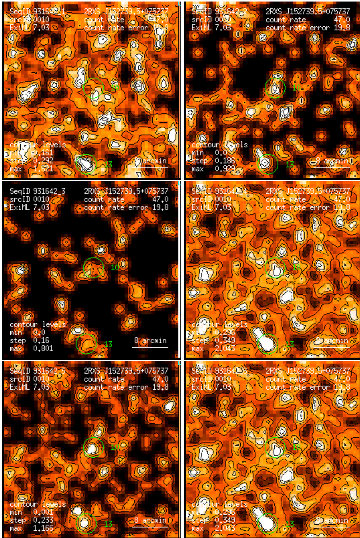
Figure 10: RASS 931642: detection 0010: band rate images, Gaussian filter: (1) PSPC channels 11 – 41, (2) 52 – 90, (3) 91 – 201, (4) 11 – 235, (5) 52 – 201, (6) 11 – 201. Broad band rates in counts/ks. Band rate contour levels in counts/ks/arcmin 2 .
