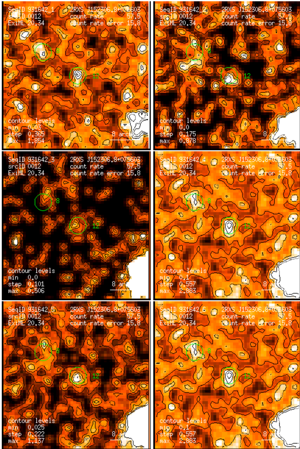
Figure 12: RASS 931642: detection 0012: band rate images, Gaussian filter: (1) PSPC channels 11 – 41, (2) 52 – 90, (3) 91 – 201, (4) 11 – 235, (5) 52 – 201, (6) 11 – 201. Broad band rates in counts/ks. Band rate contour levels in counts/ks/arcmin 2 .
