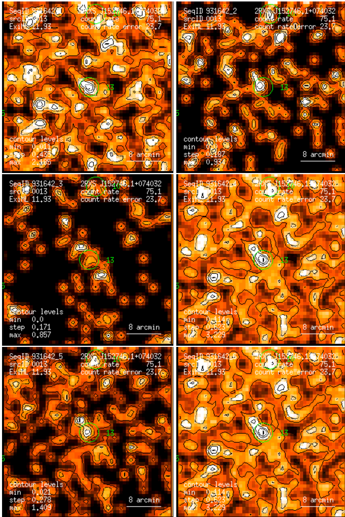
Figure 13: RASS 931642: detection 0013: band rate images, Gaussian filter: (1) PSPC channels 11 – 41, (2) 52 – 90, (3) 91 – 201, (4) 11 – 235, (5) 52 – 201, (6) 11 – 201. Broad band rates in counts/ks. Band rate contour levels in counts/ks/arcmin 2 .
