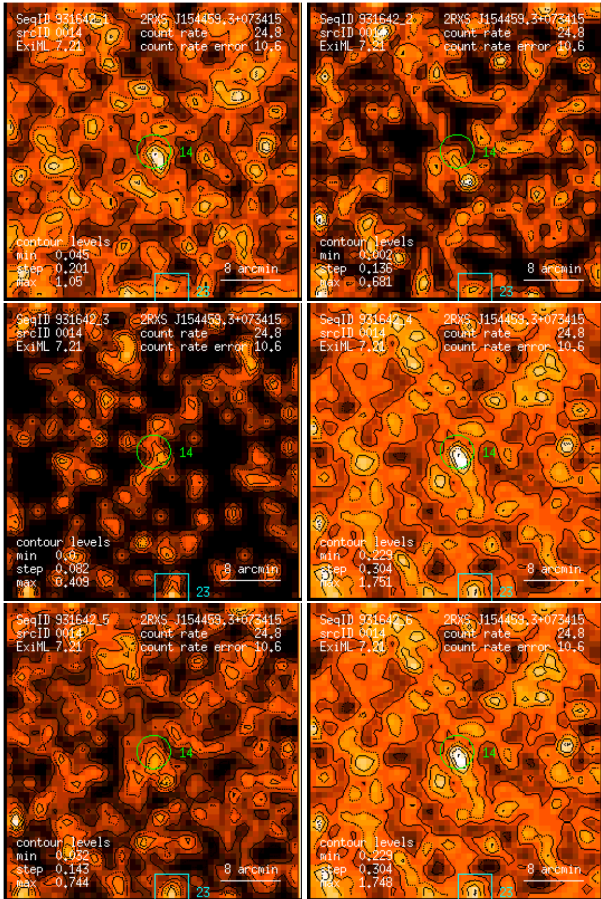
Figure 14: RASS 931642: detection 0014: band rate images, Gaussian filter: (1) PSPC channels 11 – 41, (2) 52 – 90, (3) 91 – 201, (4) 11 – 235, (5) 52 – 201, (6) 11 – 201. Broad band rates in counts/ks. Band rate contour levels in counts/ks/arcmin 2 .
