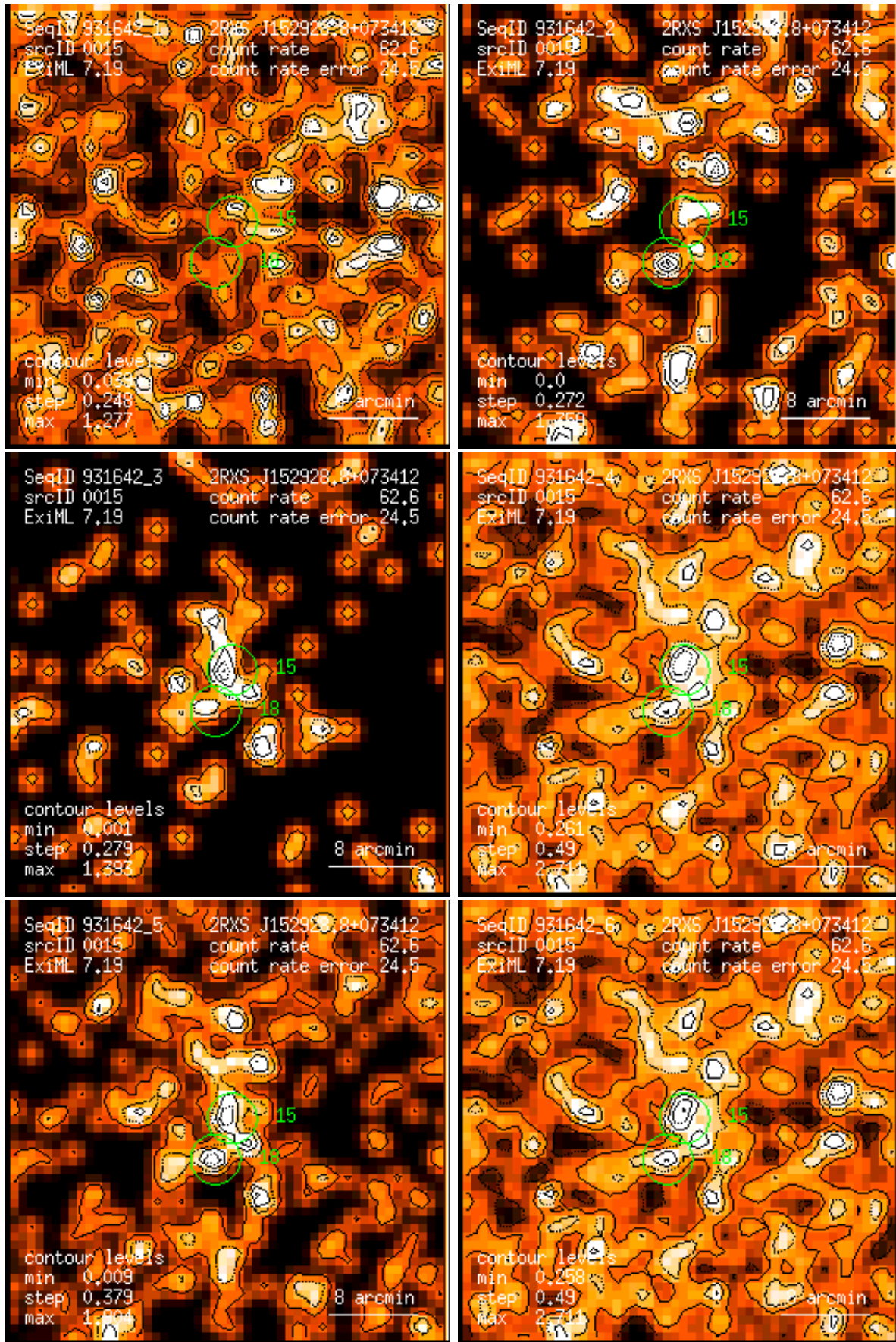
Figure 15: RASS 931642: detection 0015: band rate images, Gaussian filter: (1) PSPC channels 11 – 41, (2) 52 – 90, (3) 91 – 201, (4) 11 – 235, (5) 52 – 201, (6) 11 – 201. Broad band rates in counts/ks. Band rate contour levels in counts/ks/arcmin 2 .
