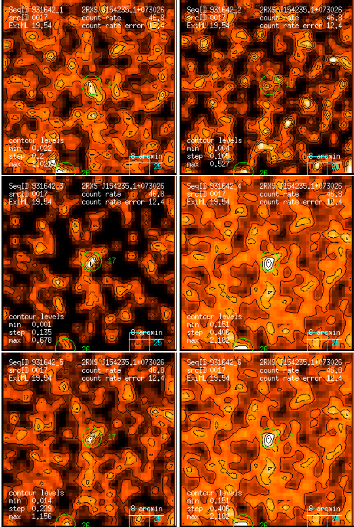
Figure 17: RASS 931642: detection 0017: band rate images, Gaussian filter: (1) PSPC channels 11 – 41, (2) 52 – 90, (3) 91 – 201, (4) 11 – 235, (5) 52 – 201, (6) 11 – 201. Broad band rates in counts/ks. Band rate contour levels in counts/ks/arcmin 2 .
