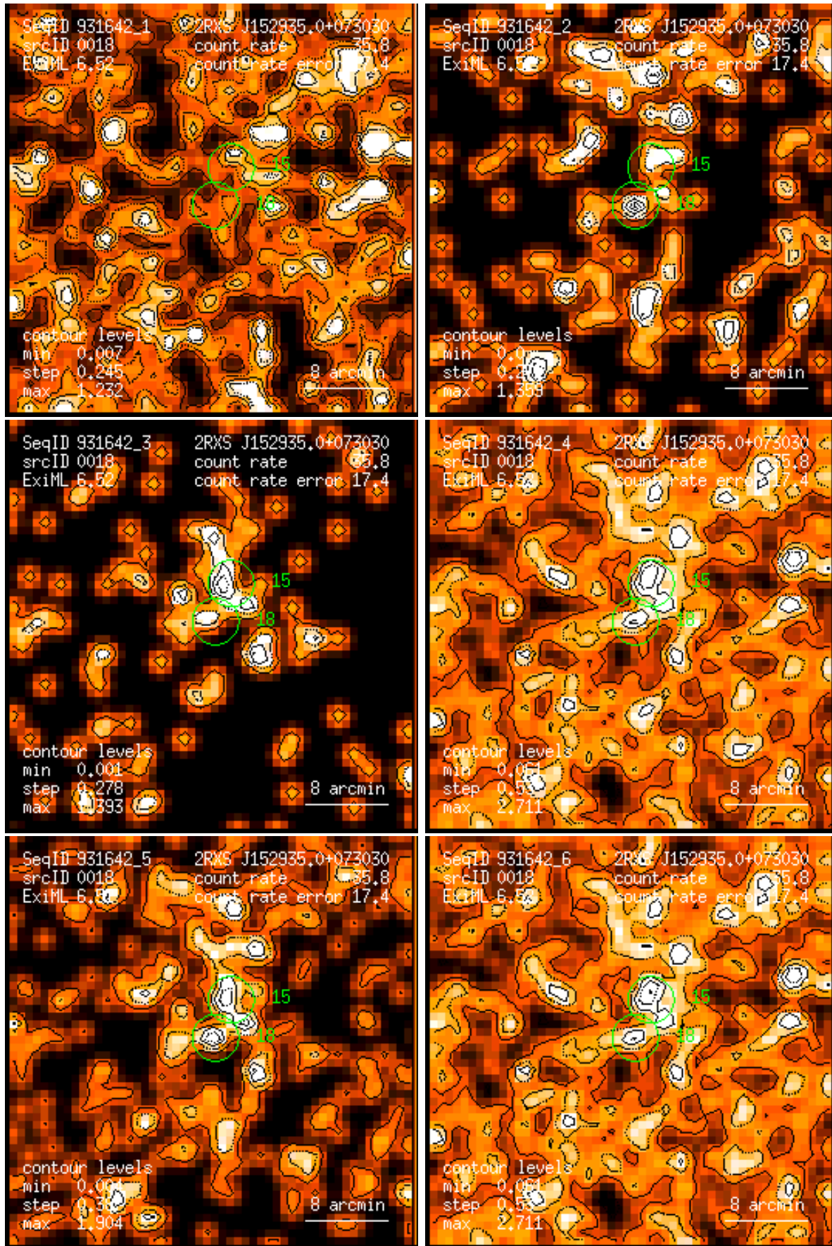
Figure 18: RASS 931642: detection 0018: band rate images, Gaussian filter: (1) PSPC channels 11 – 41, (2) 52 – 90, (3) 91 – 201, (4) 11 – 235, (5) 52 – 201, (6) 11 – 201. Broad band rates in counts/ks. Band rate contour levels in counts/ks/arcmin 2 .
