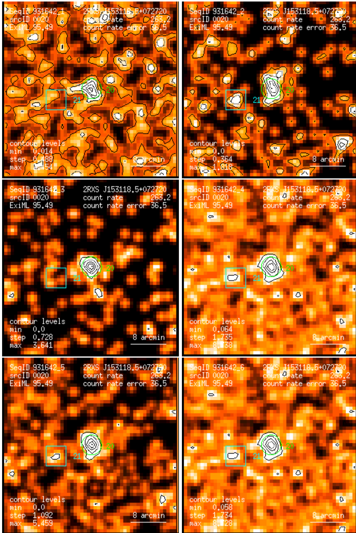
Figure 20: RASS 931642: detection 0020: band rate images, Gaussian filter: (1) PSPC channels 11 – 41, (2) 52 – 90, (3) 91 – 201, (4) 11 – 235, (5) 52 – 201, (6) 11 – 201. Broad band rates in counts/ks. Band rate contour levels in counts/ks/arcmin 2 .
