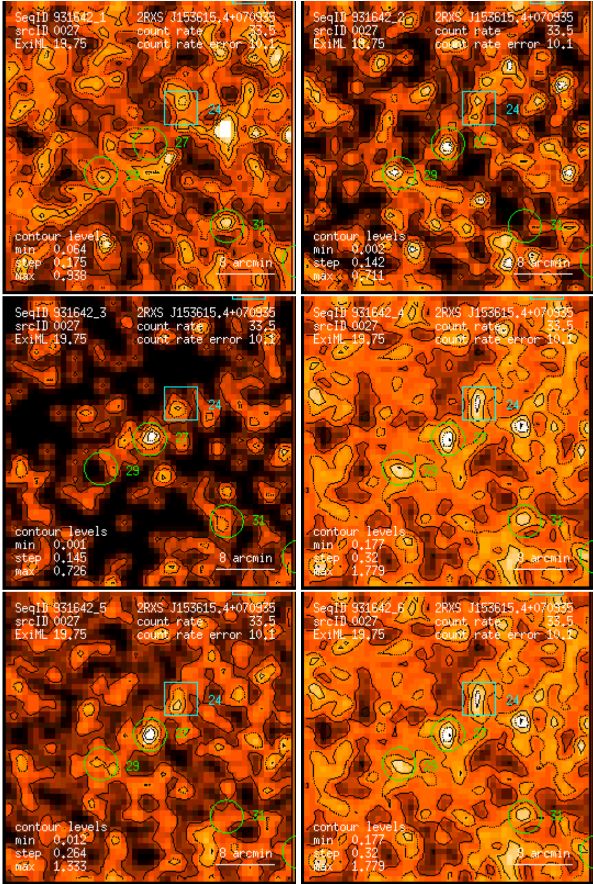
Figure 27: RASS 931642: detection 0027: band rate images, Gaussian filter: (1) PSPC channels 11 – 41, (2) 52 – 90, (3) 91 – 201, (4) 11 – 235, (5) 52 – 201, (6) 11 – 201. Broad band rates in counts/ks. Band rate contour levels in counts/ks/arcmin 2 .
