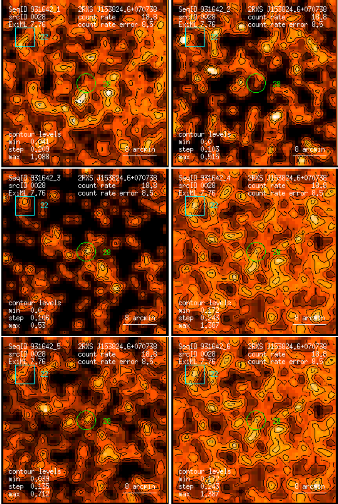
Figure 28: RASS 931642: detection 0028: band rate images, Gaussian filter: (1) PSPC channels 11 – 41, (2) 52 – 90, (3) 91 – 201, (4) 11 – 235, (5) 52 – 201, (6) 11 – 201. Broad band rates in counts/ks. Band rate contour levels in counts/ks/arcmin 2 .
