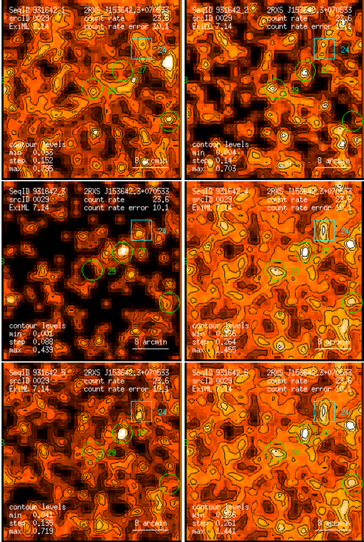
Figure 29: RASS 931642: detection 0029: band rate images, Gaussian filter: (1) PSPC channels 11 – 41, (2) 52 – 90, (3) 91 – 201, (4) 11 – 235, (5) 52 – 201, (6) 11 – 201. Broad band rates in counts/ks. Band rate contour levels in counts/ks/arcmin 2 .
