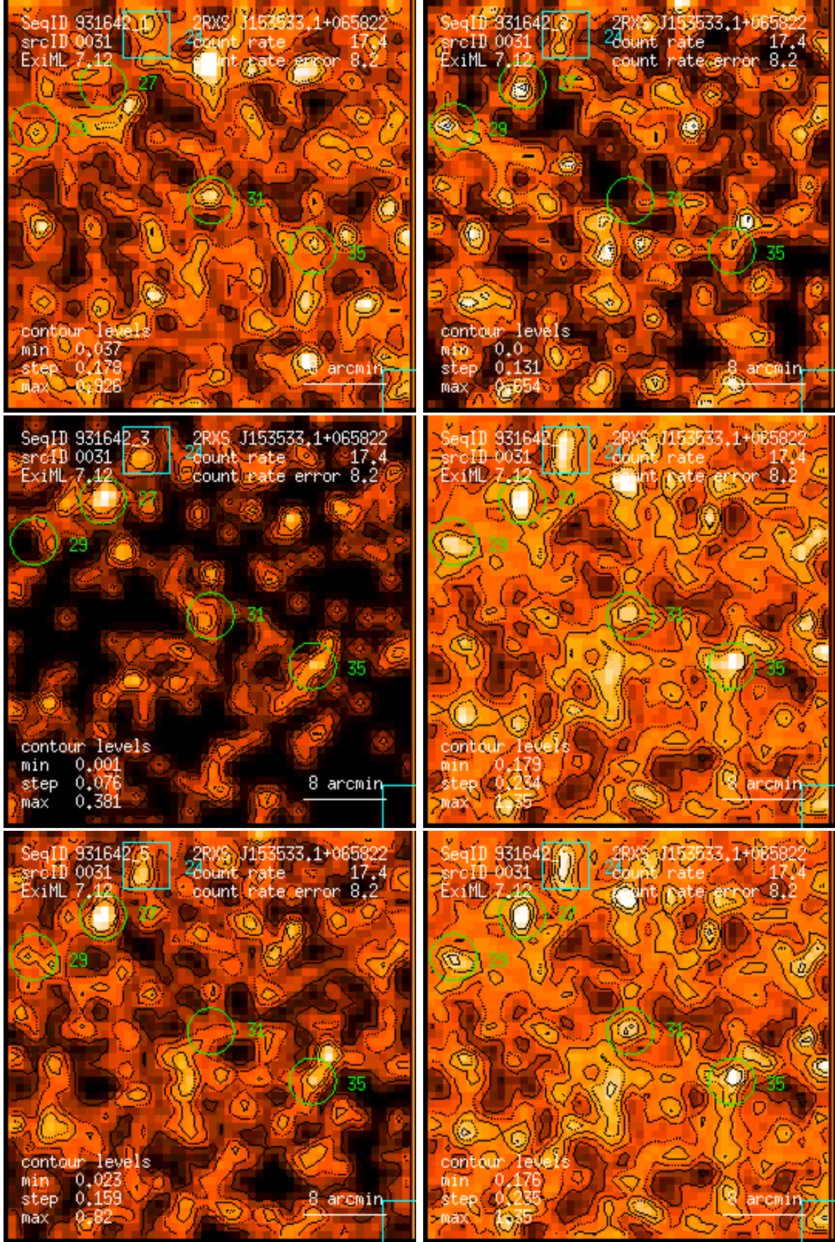
Figure 31: RASS 931642: detection 0031: band rate images, Gaussian filter: (1) PSPC channels 11 – 41, (2) 52 – 90, (3) 91 – 201, (4) 11 – 235, (5) 52 – 201, (6) 11 – 201. Broad band rates in counts/ks. Band rate contour levels in counts/ks/arcmin 2 .
