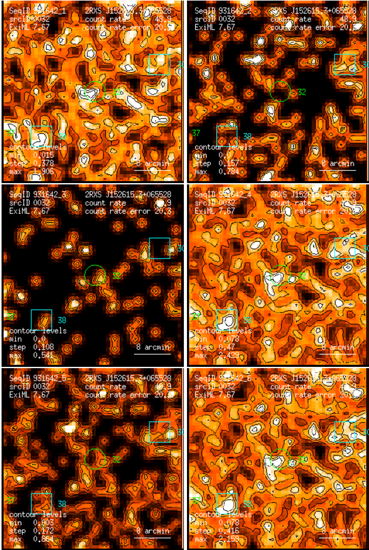
Figure 32: RASS 931642: detection 0032: band rate images, Gaussian filter: (1) PSPC channels 11 – 41, (2) 52 – 90, (3) 91 – 201, (4) 11 – 235, (5) 52 – 201, (6) 11 – 201. Broad band rates in counts/ks. Band rate contour levels in counts/ks/arcmin 2 .
