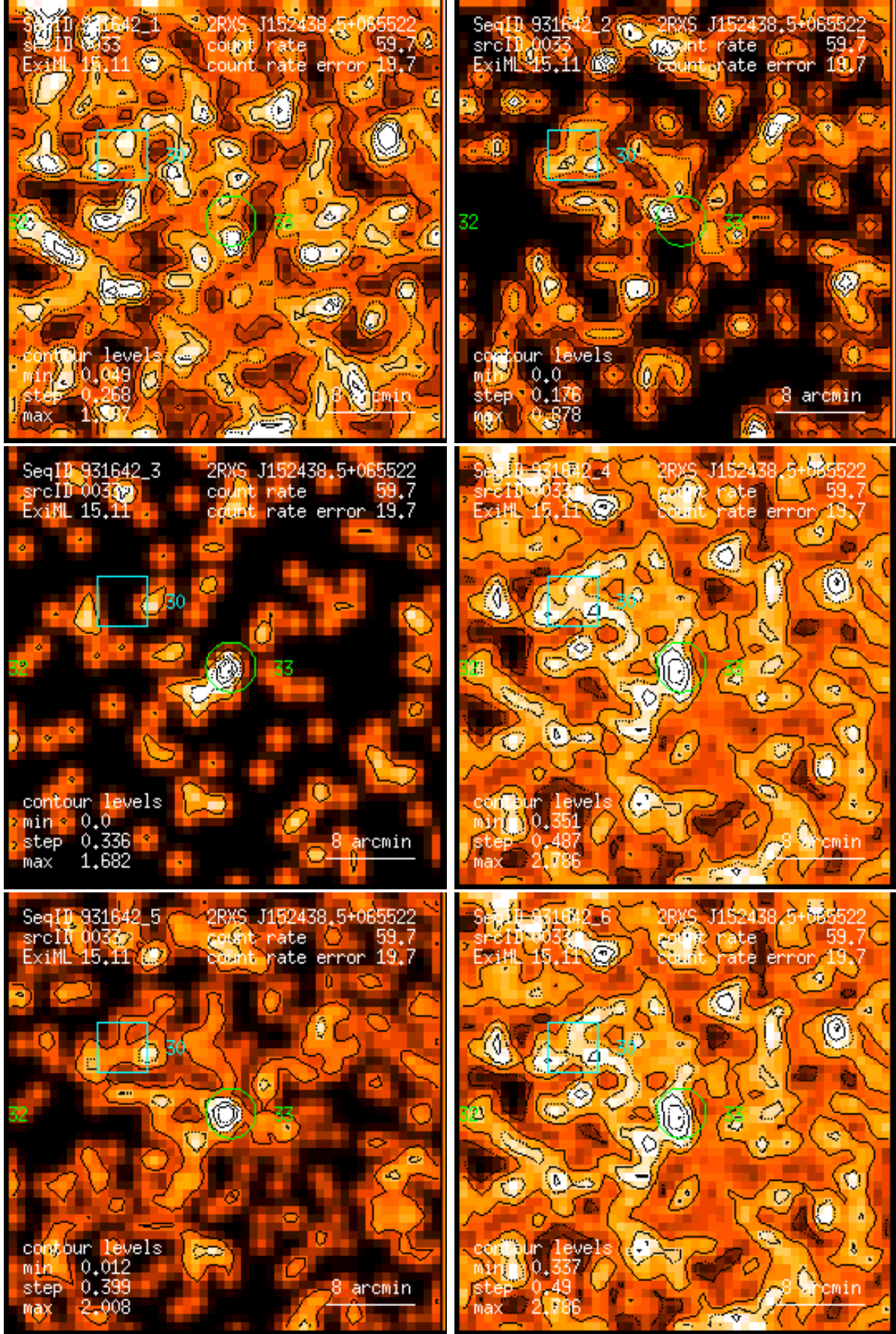
Figure 33: RASS 931642: detection 0033: band rate images, Gaussian filter: (1) PSPC channels 11 – 41, (2) 52 – 90, (3) 91 – 201, (4) 11 – 235, (5) 52 – 201, (6) 11 – 201. Broad band rates in counts/ks. Band rate contour levels in counts/ks/arcmin 2 .
