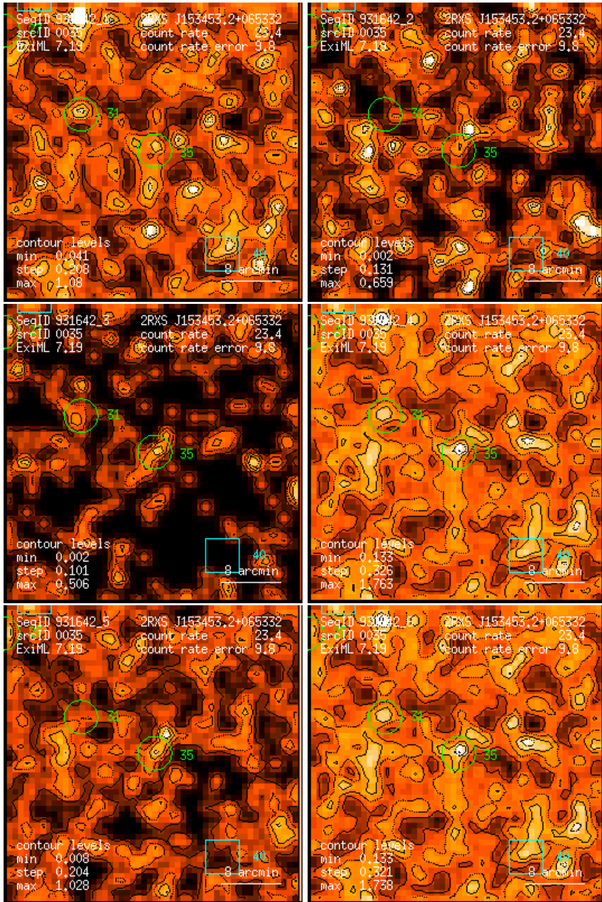
Figure 35: RASS 931642: detection 0035: band rate images, Gaussian filter: (1) PSPC channels 11 – 41, (2) 52 – 90, (3) 91 – 201, (4) 11 – 235, (5) 52 – 201, (6) 11 – 201. Broad band rates in counts/ks. Band rate contour levels in counts/ks/arcmin 2 .
