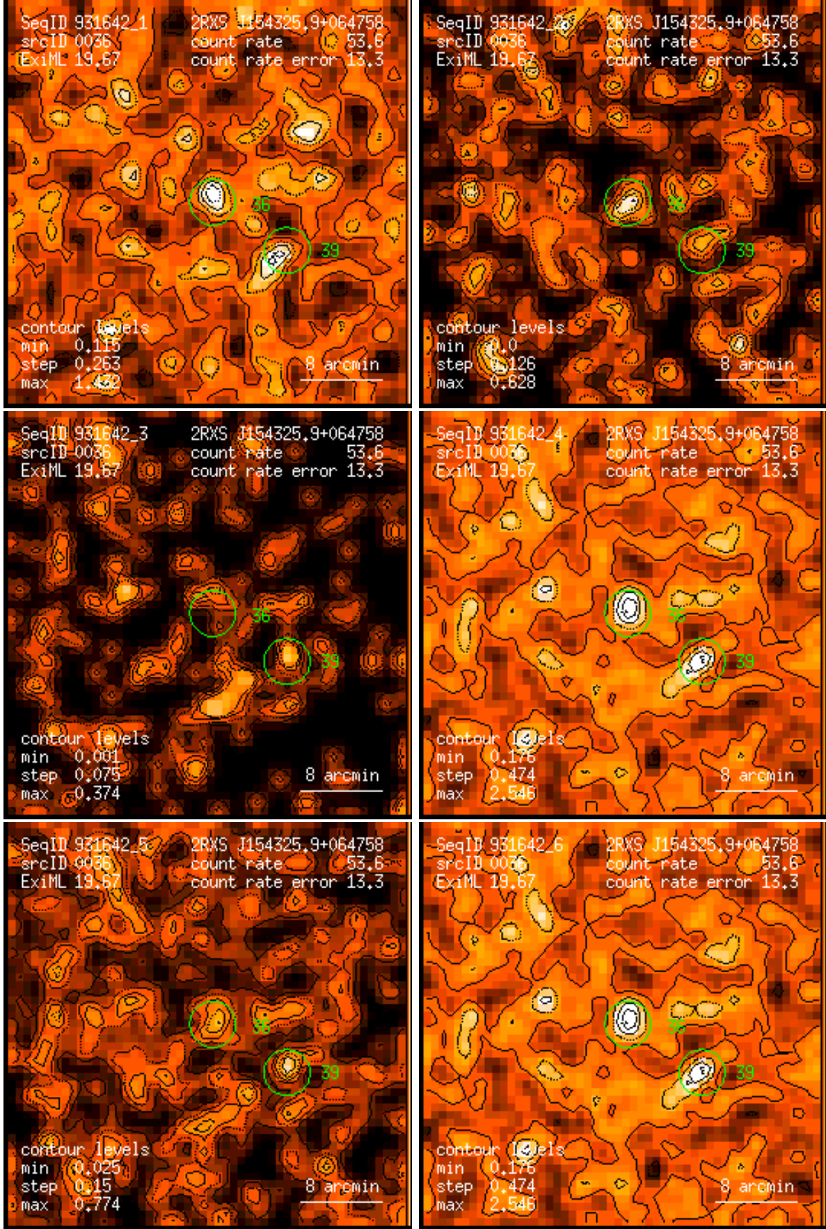
Figure 36: RASS 931642: detection 0036: band rate images, Gaussian filter: (1) PSPC channels 11 – 41, (2) 52 – 90, (3) 91 – 201, (4) 11 – 235, (5) 52 – 201, (6) 11 – 201. Broad band rates in counts/ks. Band rate contour levels in counts/ks/arcmin 2 .
