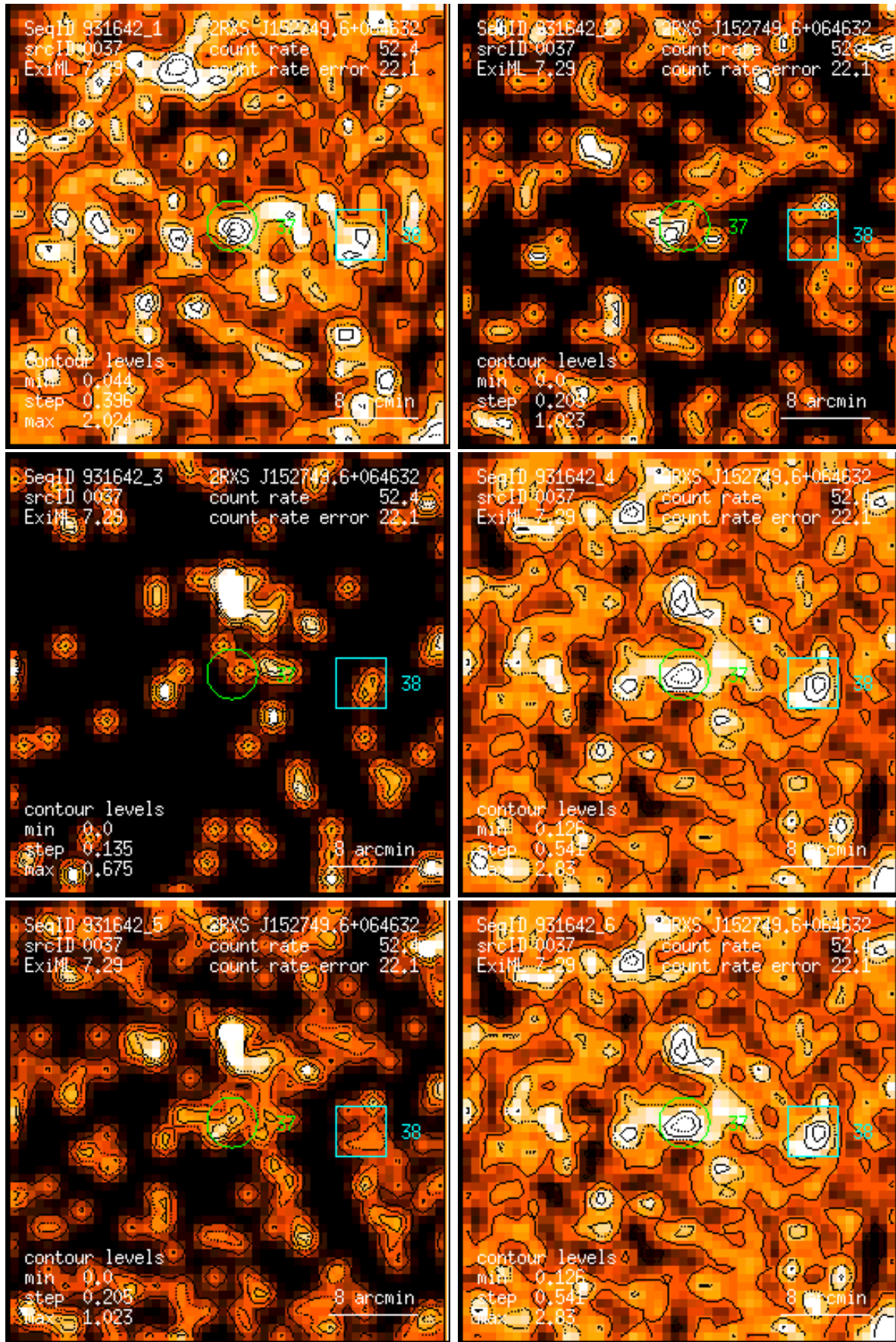
Figure 37: RASS 931642: detection 0037: band rate images, Gaussian filter: (1) PSPC channels 11 – 41, (2) 52 – 90, (3) 91 – 201, (4) 11 – 235, (5) 52 – 201, (6) 11 – 201. Broad band rates in counts/ks. Band rate contour levels in counts/ks/arcmin 2 .
