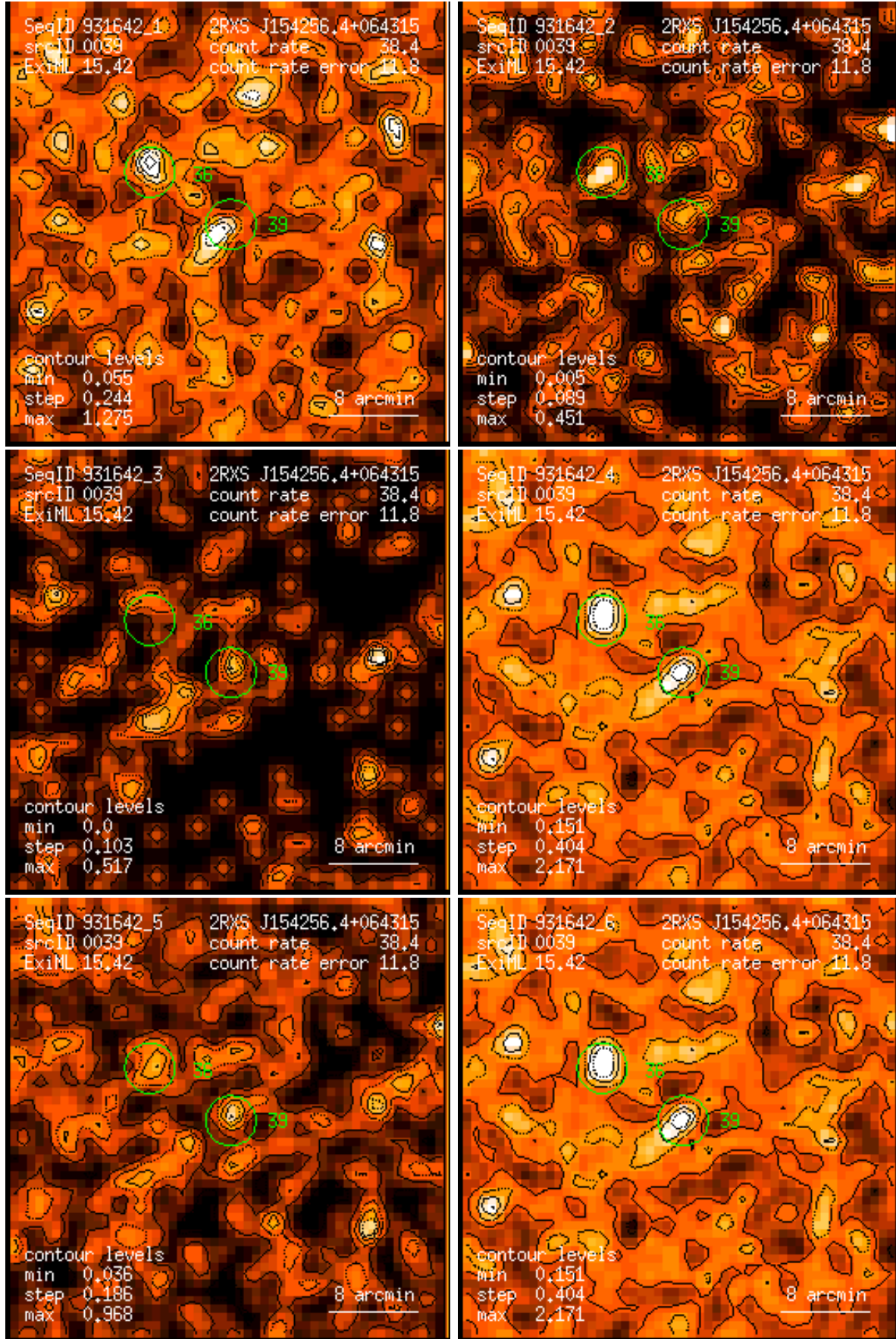
Figure 39: RASS 931642: detection 0039: band rate images, Gaussian filter: (1) PSPC channels 11 – 41, (2) 52 – 90, (3) 91 – 201, (4) 11 – 235, (5) 52 – 201, (6) 11 – 201. Broad band rates in counts/ks. Band rate contour levels in counts/ks/arcmin 2 .
