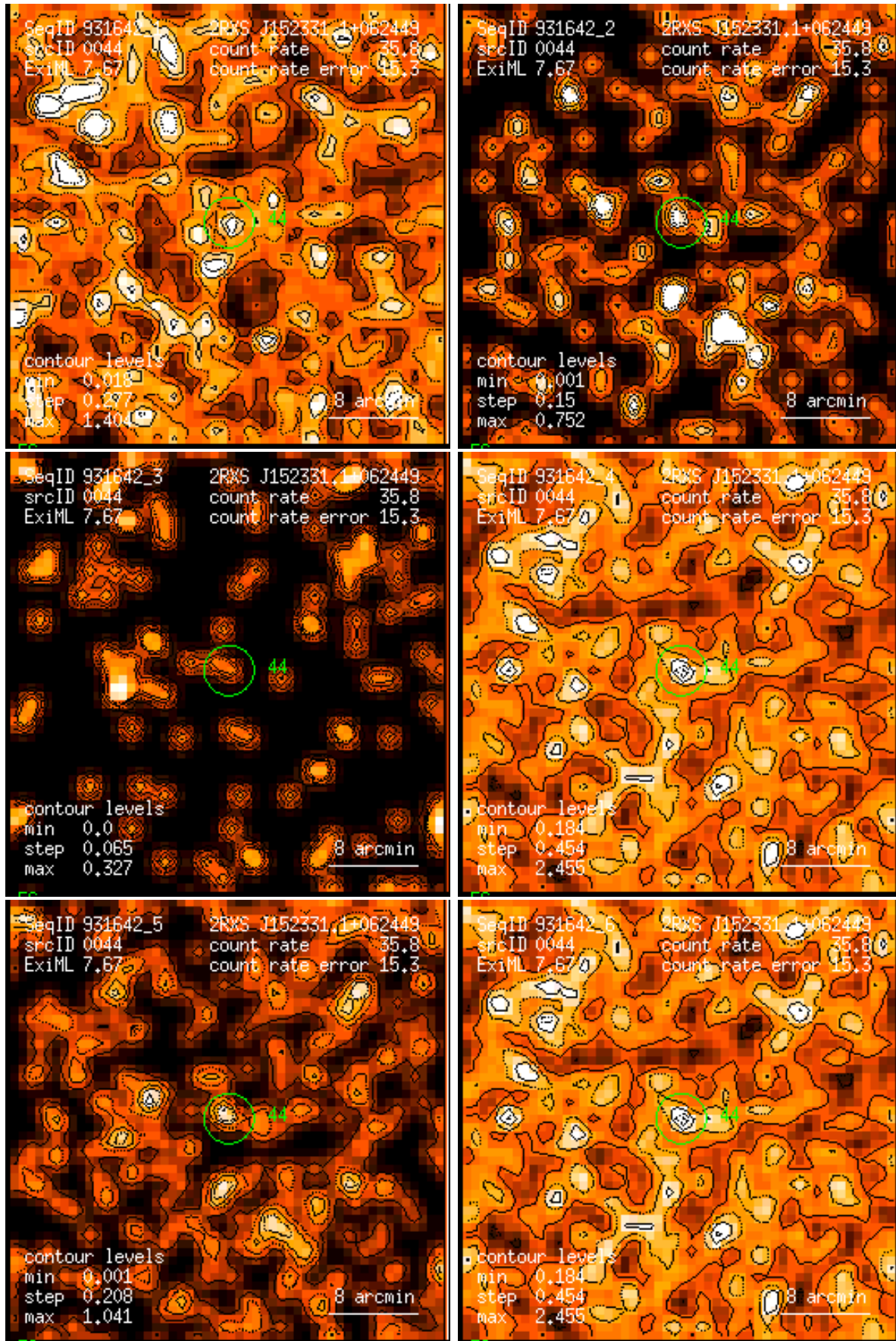
Figure 44: RASS 931642: detection 0044: band rate images, Gaussian filter: (1) PSPC channels 11 – 41, (2) 52 – 90, (3) 91 – 201, (4) 11 – 235, (5) 52 – 201, (6) 11 – 201. Broad band rates in counts/ks. Band rate contour levels in counts/ks/arcmin 2 .
