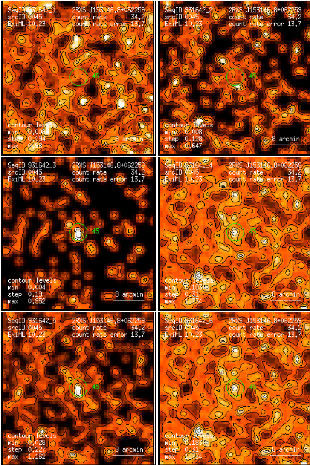
Figure 45: RASS 931642: detection 0045: band rate images, Gaussian filter: (1) PSPC channels 11 – 41, (2) 52 – 90, (3) 91 – 201, (4) 11 – 235, (5) 52 – 201, (6) 11 – 201. Broad band rates in counts/ks. Band rate contour levels in counts/ks/arcmin 2 .
