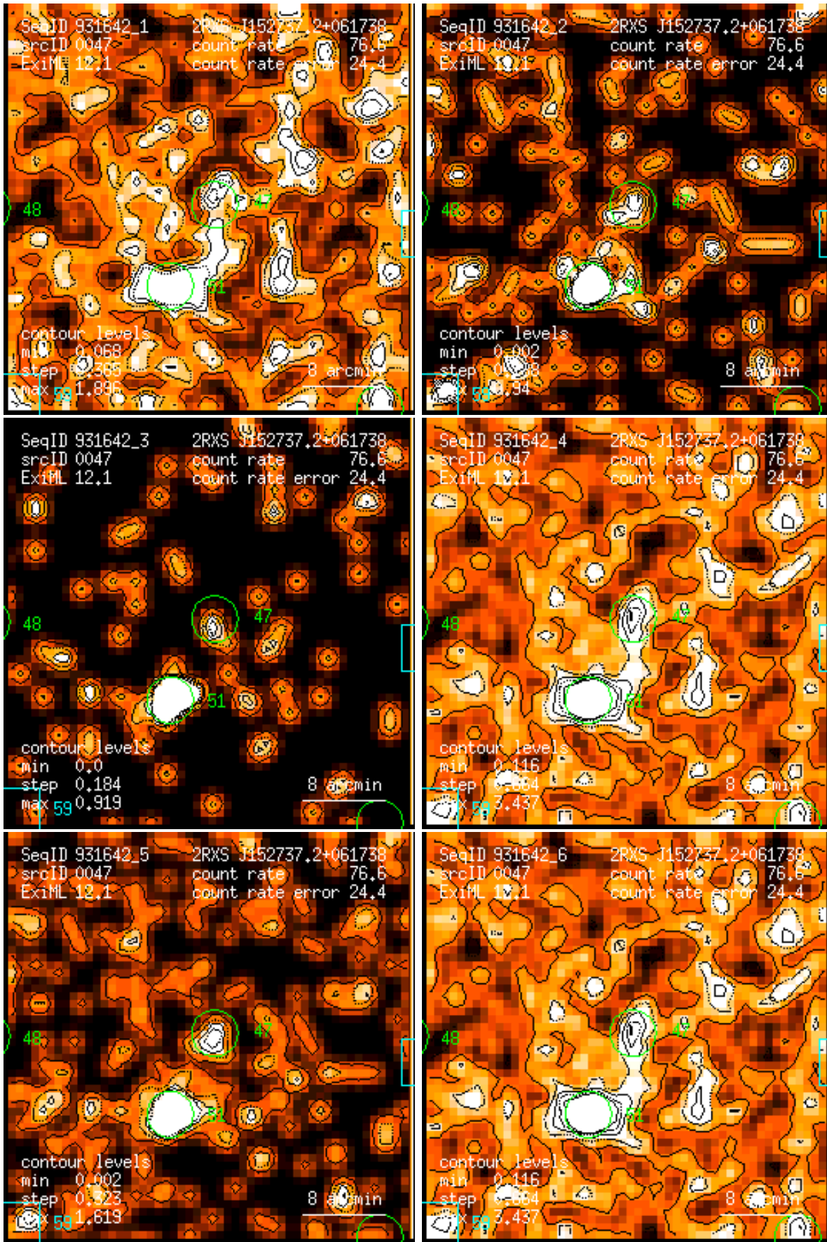
Figure 47: RASS 931642: detection 0047: band rate images, Gaussian filter: (1) PSPC channels 11 – 41, (2) 52 – 90, (3) 91 – 201, (4) 11 – 235, (5) 52 – 201, (6) 11 – 201. Broad band rates in counts/ks. Band rate contour levels in counts/ks/arcmin 2 .
