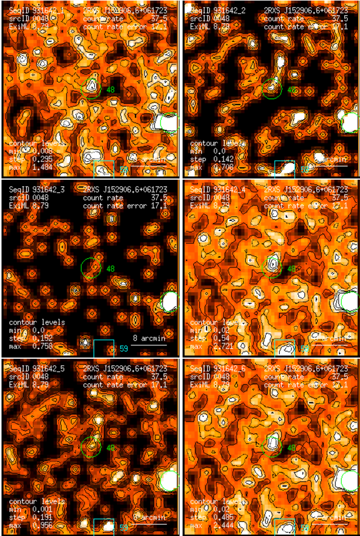
Figure 48: RASS 931642: detection 0048: band rate images, Gaussian filter: (1) PSPC channels 11 – 41, (2) 52 – 90, (3) 91 – 201, (4) 11 – 235, (5) 52 – 201, (6) 11 – 201. Broad band rates in counts/ks. Band rate contour levels in counts/ks/arcmin 2 .
