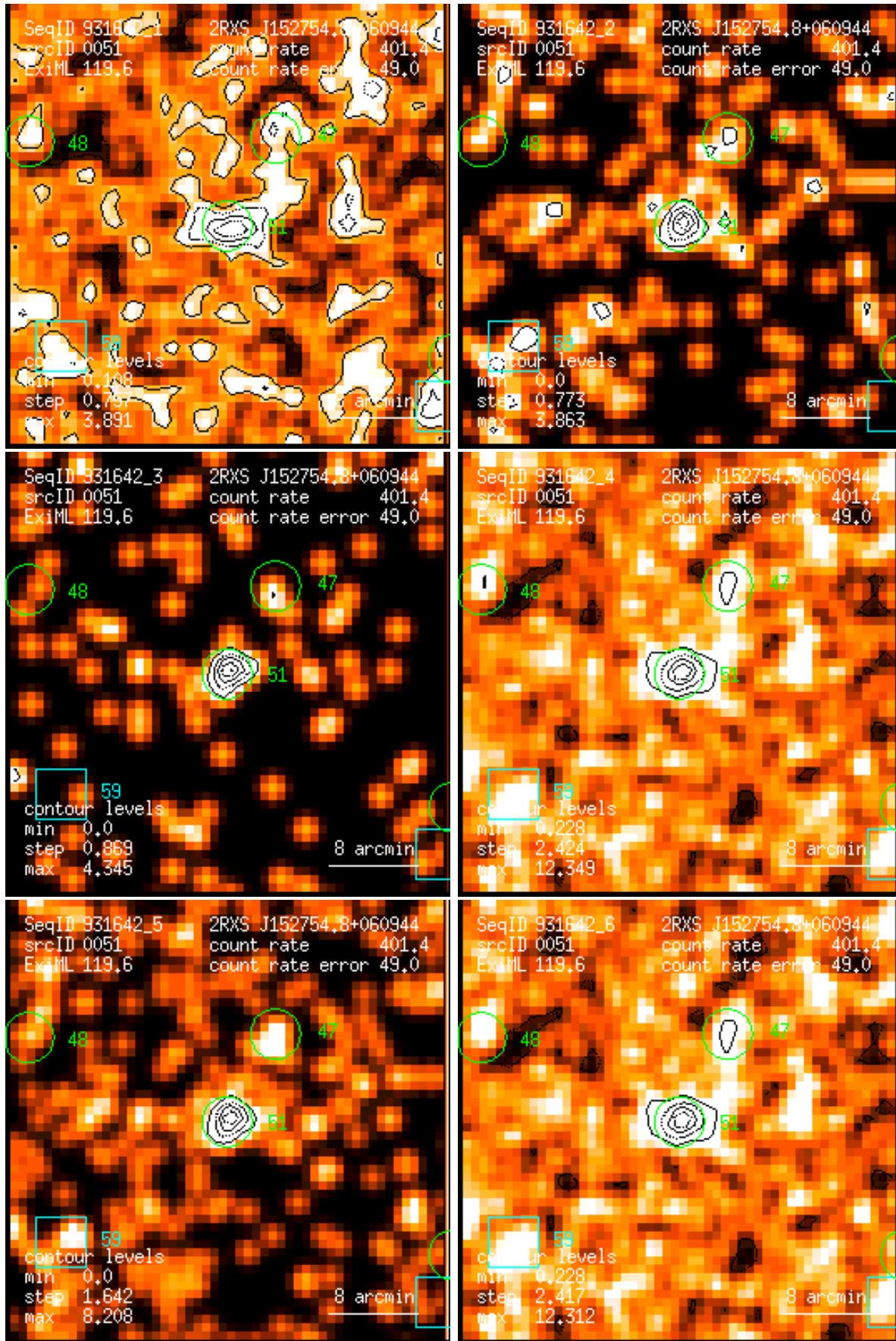
Figure 51: RASS 931642: detection 0051: band rate images, Gaussian filter: (1) PSPC channels 11 – 41, (2) 52 – 90, (3) 91 – 201, (4) 11 – 235, (5) 52 – 201, (6) 11 – 201. Broad band rates in counts/ks. Band rate contour levels in counts/ks/arcmin 2 .
