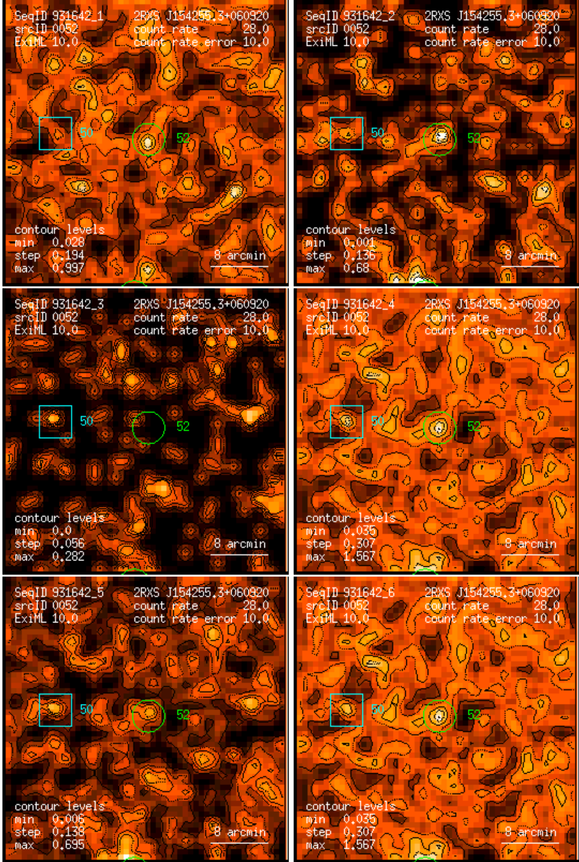
Figure 52: RASS 931642: detection 0052: band rate images, Gaussian filter: (1) PSPC channels 11 – 41, (2) 52 – 90, (3) 91 – 201, (4) 11 – 235, (5) 52 – 201, (6) 11 – 201. Broad band rates in counts/ks. Band rate contour levels in counts/ks/arcmin 2 .
