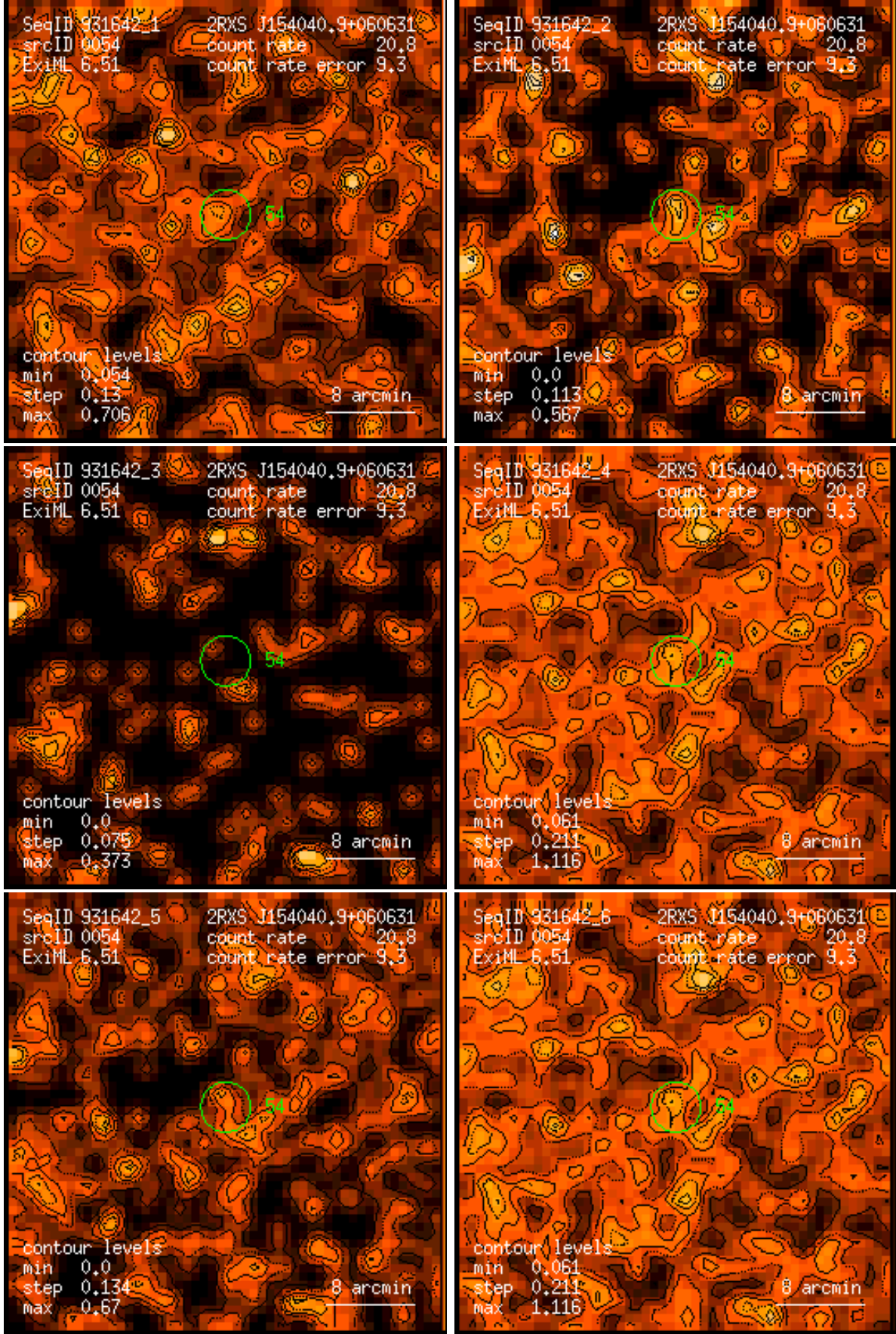
Figure 54: RASS 931642: detection 0054: band rate images, Gaussian filter: (1) PSPC channels 11 – 41, (2) 52 – 90, (3) 91 – 201, (4) 11 – 235, (5) 52 – 201, (6) 11 – 201. Broad band rates in counts/ks. Band rate contour levels in counts/ks/arcmin 2 .
