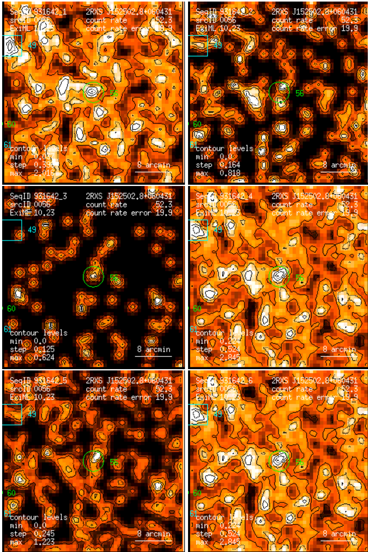
Figure 56: RASS 931642: detection 0056: band rate images, Gaussian filter: (1) PSPC channels 11 – 41, (2) 52 – 90, (3) 91 – 201, (4) 11 – 235, (5) 52 – 201, (6) 11 – 201. Broad band rates in counts/ks. Band rate contour levels in counts/ks/arcmin 2 .
